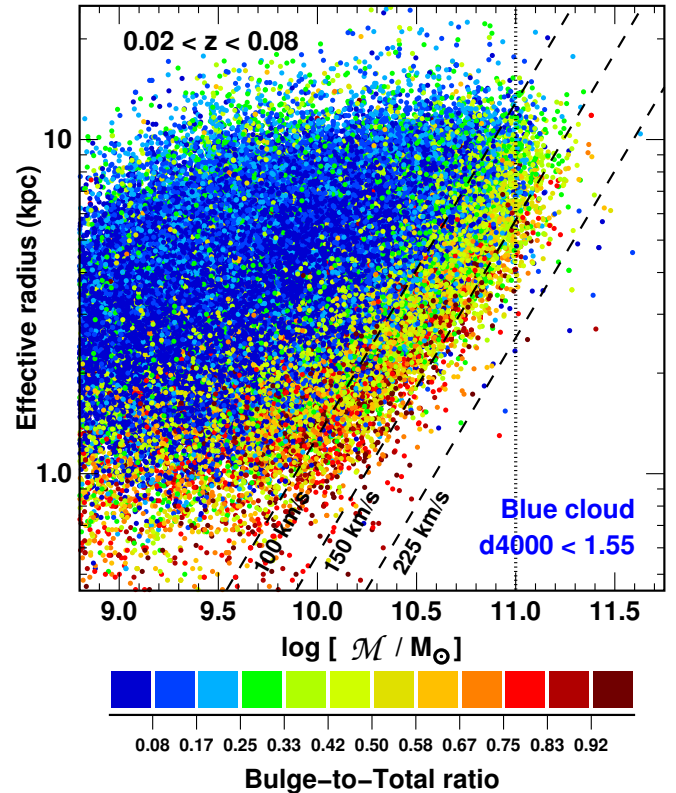
Fig. B.1. Size-mass relation of SDSS blue-cloud galaxies ( d4000 < 1.55 ) in the local Universe ( 0.02 \leq z < 0.08 ). Galaxies are colour coded according to their bulge-to-total ( B/T ) ratio derived by Simard et al. (2011).
