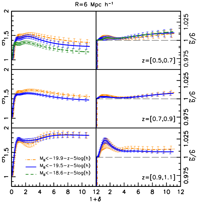
Fig. 10. Left: second-order moment \hat{b}(\delta) of the reconstructed mean biasing functions shown in Fig. 7. The cell size is R = 6 h^{-1} Mpc. Different line styles and colours indicate different luminosity cuts listed in the plot. The redshift ranges and colour codes are the same as in Fig. 7. Error bars represent the 1\sigma scatter among the mocks. Right: similar plots showing the non-linear bias parameter \tilde{b}/\hat{b}(\delta) . A horizontal offset \delta = 0.015 was applied to avoid overlapping error bars. All curves are plotted out to \delta_{\text{MAX}} .
