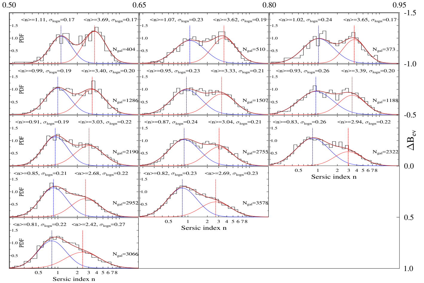
Fig. 5. Sérsic index distribution (black histograms) for different redshift ( from left to right ) and \Delta B_{\text{ev}} luminosity bins ( from top to bottom ). The blue and red solid lines show the Gaussian fits to the disc-like and spheroid-like populations, respectively. The vertical dashed lines mark the central values of each Gaussian. The sum of the two Gaussian fits is shown as a solid brown line. The central values \langle n \rangle of the Gauss functions, their 1\sigma widths, and the total number of galaxies in each bin are shown in each panel.
