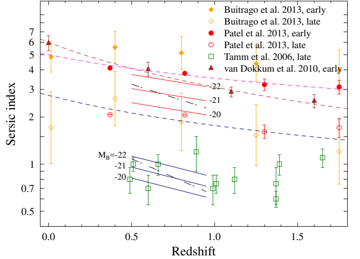
Fig. 6. Sérsic index – redshift relation: VIPERS results are presented as red and blue solid lines for spheroid- and disc-like galaxies, respectively, for three values of B -band absolute magnitude. Patel et al. (2013)’s results for quiescent and star-forming objects with \log(M/M_\odot) > 10.5 are shown as red filled and empty circles and dashed magenta and blue lines. The relation found by van Dokkum et al. (2010) for a constant co-moving number density sample is plotted in brown (short-dashed line and triangles). Buitrago et al. (2013)’s results for a sample visually classified into early- and late-type galaxies is shown as orange filled and empty diamonds, while disc-galaxies measured by Tamm & Tenjes (2006) are represented by green squares. The dot-dashed lines show n(z) relation corresponding to the disk-like and spheroidal galaxies, only for M_B = -21 mag, obtained from the 2D analysis presented in Sect. 6.
