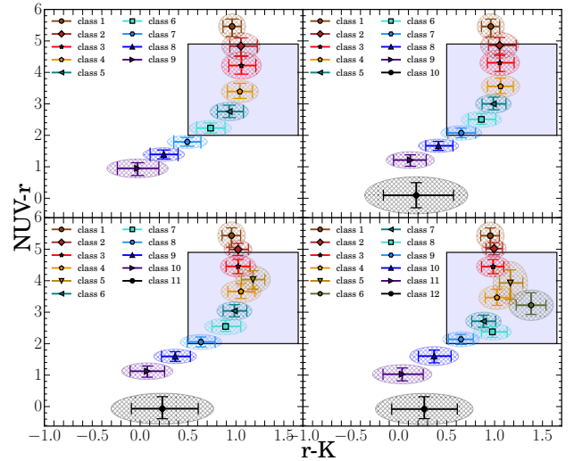
Fig. 1. NUVrK diagrams of FEM classes 9–12. The optimal number of classes was found to be 12. The error bars correspond to the first and the third quartile of the galaxy colour distribution, while the two half axes of the ellipses correspond to the median absolute deviation.
