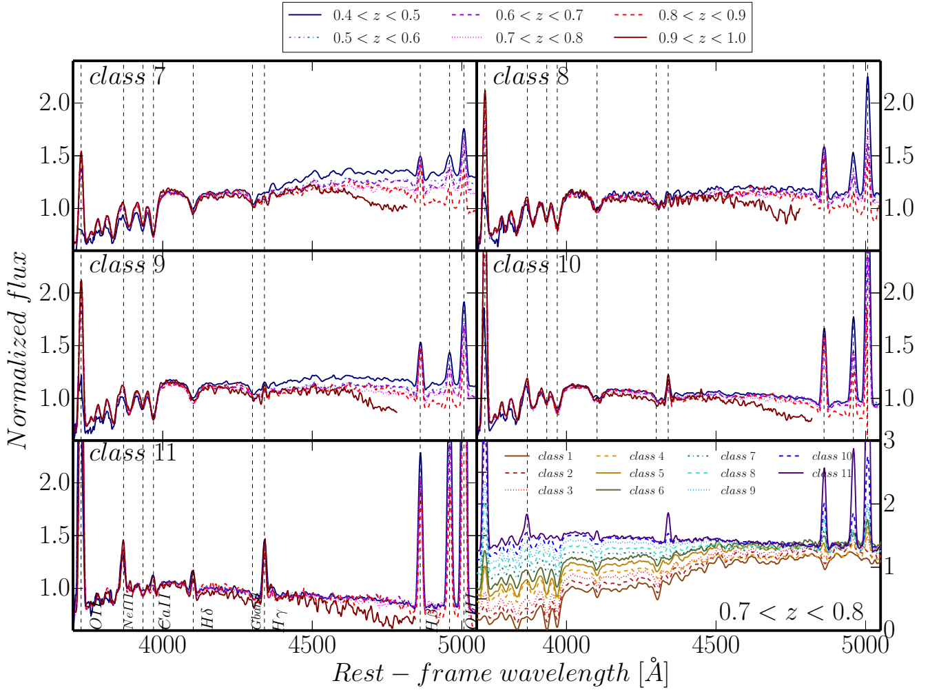
Fig. 9. Stacked spectra of VIPERS galaxies among FEM classes 7–11 in different redshift bins. Rest-frame composite spectra were normalised in the region 3600 < \lambda < 4500 \text{ \AA} . The most prominent spectral lines are marked with vertical solid lines with labels. The last panel shows stacked spectra of FEM classes 1–11 in redshift bin 0.7 < z < 0.8 .
