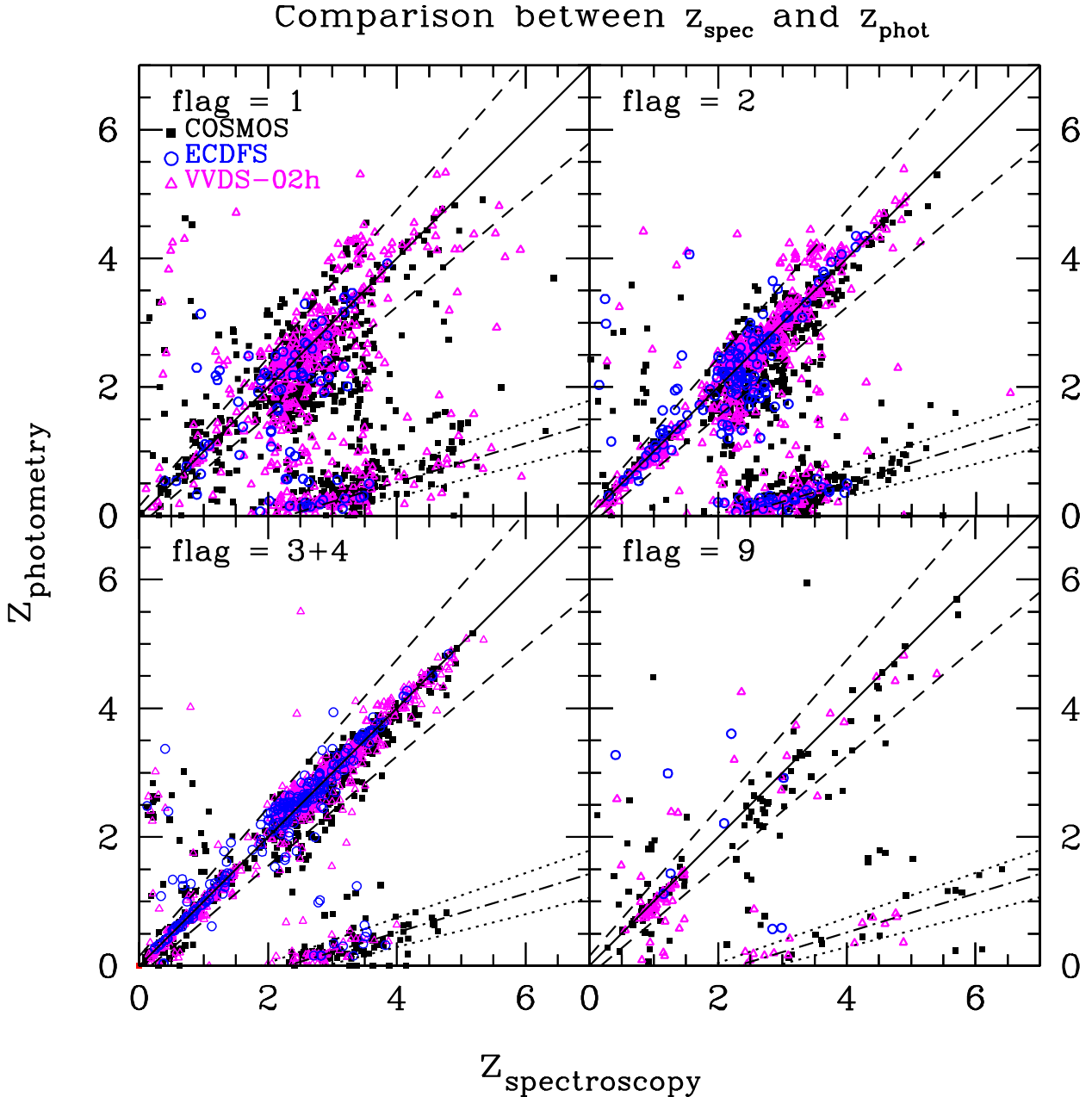
Fig. 11. A posteriori comparison between VUDS spectroscopic redshifts and the SED-derived photometric redshifts using the Le Phare code. Top-left: VUDS galaxies with spectroscopic flag 1 ( \approx 50 – 70\% reliable), top right: VUDS galaxies with spectroscopic flags 2 ( \approx 75 – 85\% reliable), bottom left: VUDS galaxies with spectroscopic flag 3 and 4 ( 95 – 100\% reliable), bottom-right: VUDS galaxies with spectroscopic flags 9 ( \approx 80\% reliable). Galaxies in the three different fields are identified as filled squares (COSMOS field), open triangles (VVDS-02h), and open circles (ECDFS). The 1:1 equality relation is drawn as a continuous line, and 15\% errors expressed as 0.15 \times (1 + z) are drawn as dashed lines. The known degeneracy of photometric redshifts between a Balmer- 4000 \text{ \AA} break and a \text{Ly}\alpha 1215 \text{ \AA} break is identified by the dotted-dashed line, with 15\% errors drawn with dotted lines.
