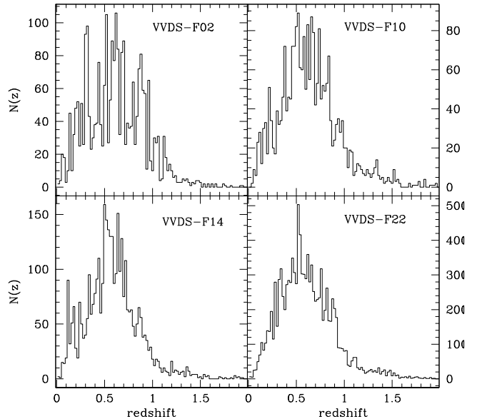
Fig. 6. Observed redshift distribution to I_{AB} = 22.5 in the four VVDS Wide fields, in redshift bins of \Delta z = 0.02 . All galaxies with quality flag between 1 to 19 have been used.
