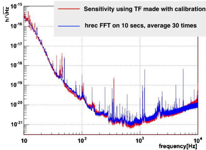
Figure 5. Comparison between a sensitivity curve obtained by the time-domain reconstruction used in Virgo and a sensitivity curve obtained using a transfer function measurement made with a complete calibration procedure.
