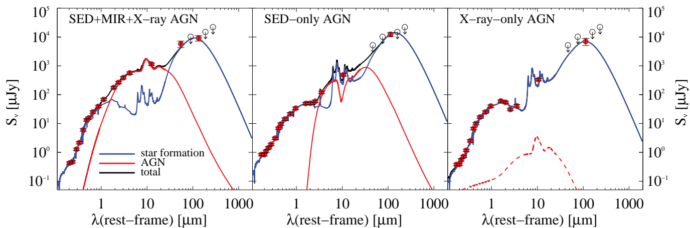
Fig. 3: Three examples of best-fit SEDs of HLAGN selected from different criteria. Coloured lines represent the corresponding best-fit templates of AGN (red), galaxy star formation (blue), and the sum of the two (black). (Left panel) AGN identified from X-rays, MIR colours, and SED fitting. (Central panel) AGN identified only from SED-fitting. (Right panel) AGN identified only from X-rays. The red dashed line indicates that the AGN component is <99\% significant on the basis of the Fisher test (see text for more details). Red circles indicate the optical to far-IR (FIR) photometry (rest-frame), while downward pointing arrows represent 3\sigma upper limits in the Herschel bands.
