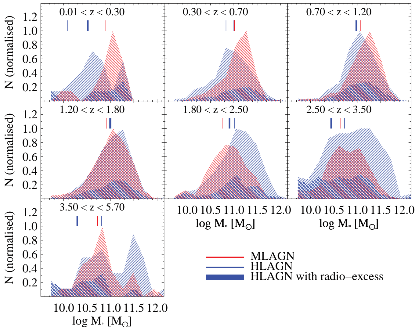
Fig. 8: Normalised distributions of M_* , as a function of redshift. Radio classes are highlighted as follows: HLAGN (blue), HLAGN subsample with radio excess (blue thicker distribution), and MLAGN (red). Vertical lines show the median value for MLAGN (red), HLAGN (blue) and their subsample with radio excess (blue thicker).
