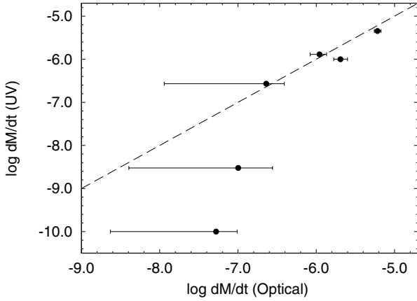
Fig. 12. Comparison of mass loss rates determined in this study using the optical spectrum with values determined from the UV spectrum. For the three objects with the lowest mass loss rates the values determined from the optical spectra correspond to upper limits.
