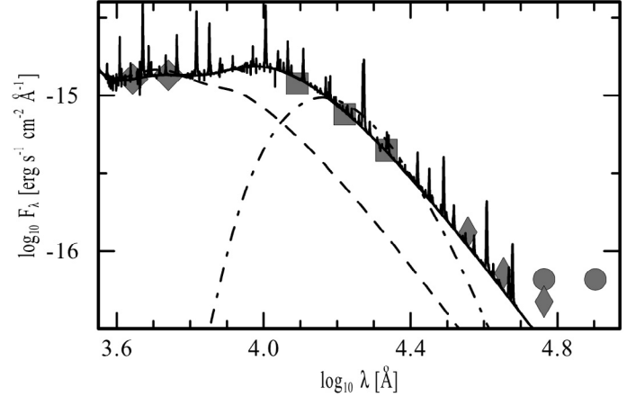
Fig. 3. Log flux vs. log wavelength. Squares: B , V , J , H , K_s photometry, Diamonds: Spitzer SAGE. Circles: Spitzer 5.8 \mu\text{m} and 8.0 \mu\text{m} from Gruendl & Chu (2009). Solid line: SED with anomalous R_V parameter. Dashed line: standard R_V parameter. Dashed-Dotted line: attempt to reproduce the NIR excess with a 1500 K black body.
