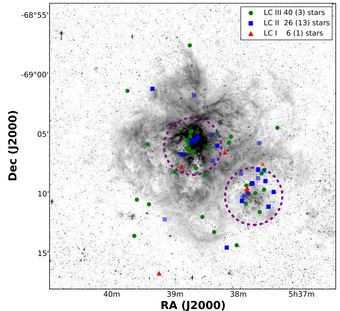
Fig. 2. Spatial distribution of the presumably single O-type stars as a function of LC. North is to the top; east is to the left. The circles define regions within 2.4' of NGC 2070 (central circle) and NGC 2060 (south-west circle). Different symbols indicate LC: III (circles), II (squares), I (triangles). Note that because of crowding a considerable fraction of the sources overlap. Lower opacities again denote sources with an ambiguous LC classification, similar as in Fig. 1.
