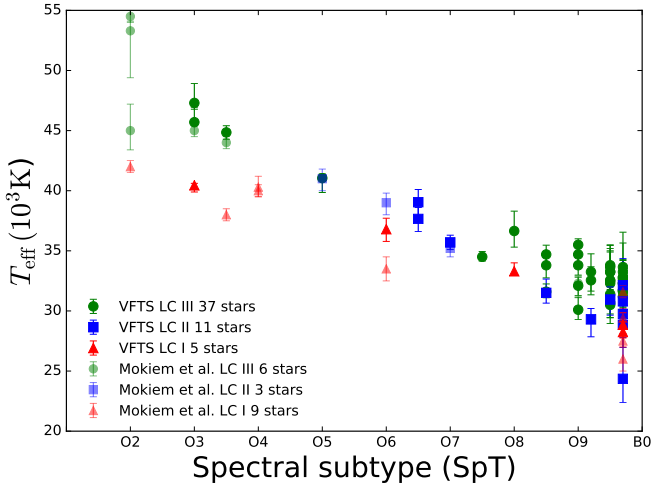
Fig. 4. Effective temperature vs. spectral subtype for the O-type with well defined LC (see main text). The lower-opacity symbols give the results for the sample of LMC stars investigated by Mokiem et al. (2007b).
