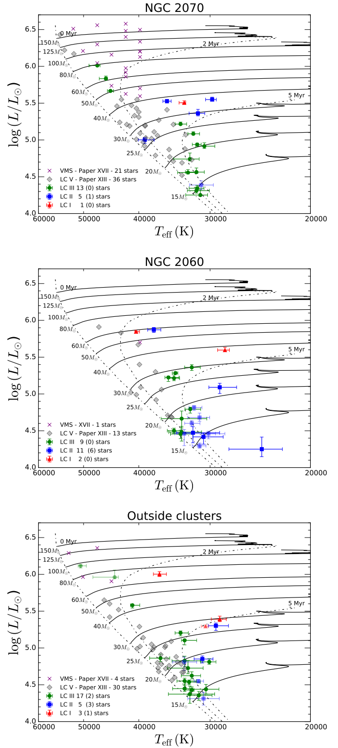
Fig. B.1. Hertzsprung-Russell diagram of the sample as a function of spatial location: NGC 2070 (upper panel), NGC 2060 (middle panel) and stars outside star-forming complexes (lower panel). Evolutionary tracks (solid lines) and isochrones (dot-dashed lines) are from stellar models initially rotating with approximately 200 \text{ km s}^{-1} (Brott et al. 2011; Köhler et al. 2015).
