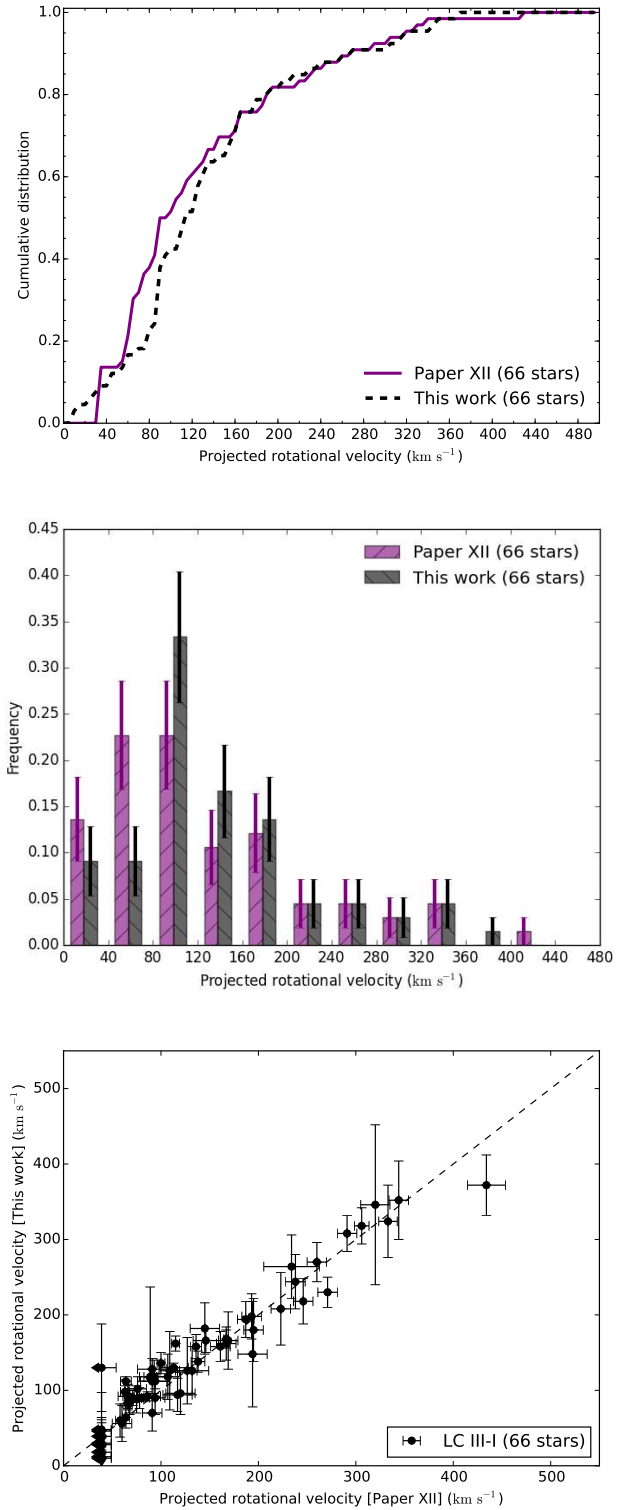
Fig. A.1. Cumulative ( upper panel ) and frequency ( middle panel ) distributions of the projected rotational velocities of the O-type LC III to I as derived here from the automated FASTWIND analysis and Paper XII. The middle panel shows Poissonian error bars. The lower panel compares the actual v_e \sin i of these two samples.
