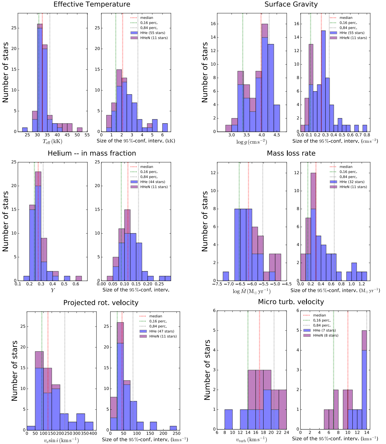
Fig. 3. Range of each fitted parameter ( left panels of each set) and accompanying range of 95% confidence interval ( right panel of each set) in the same unit. Colors have been used to differentiate between stars that have been analyzed using hydrogen and helium lines (HHe) and those for which also nitrogen lines (HHeN) were considered (see also Sect. 3.1). The distributions exclude stars for which only upper/lower limits could be determined, hence the number of stars shown in a panel depends on the parameter that is investigated. In each panel, the median value and the 16th and 84th percentiles are shown using vertical lines.
