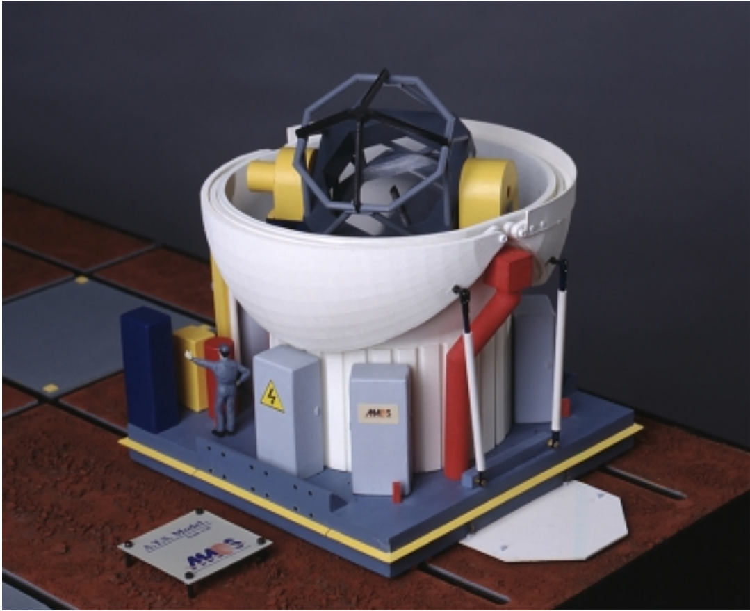
Figure 4. A model of an Auxiliary Telescope during Observations. The 1.8-m telescope (with an Alt-Az mount like the Unit Telescopes) is rigidly anchored to the ground by means of a special interface. The light is directed via the Coudé Optical Train to the bottom of the Telescope. From the Coudé Relay Optics it is sent to the underground Delay Line Tunnel
