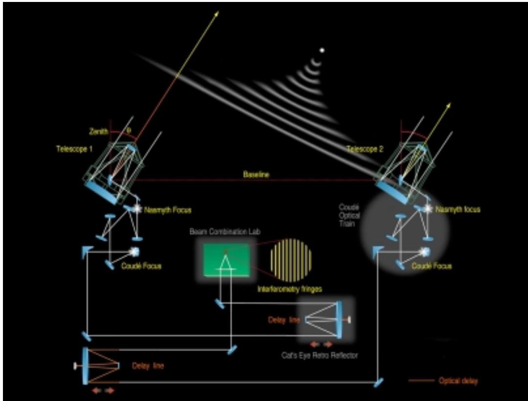
Figure 2. The optical layout of the VLTI with two telescopes. The telescopes represent both UTs and ATs that have the same optical design. The Coudé Optical Trains are the mirrors after the tertiary mirror up to the Coudé Focus. The mirrors just before and just after the Delay Lines are called the transfer optics. Two Delay Lines are shown to demonstrate the principle of operation. The VLTI laboratory is represented by the beam combining lens forming fringes.
