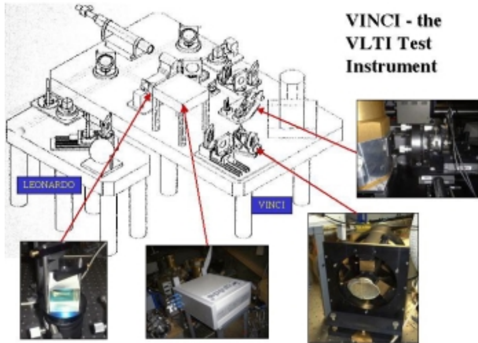
Figure 6. The concept of the VLTI commissioning instrument VINCI. The beam combining unit, VINCI, and the reference source unit, LEONARDO, are placed on individual tables. Their respective positions in the VLTI Laboratory are shown in Fig. 2. The main elements on the Vinci table are the fiber beam combiner and the dewar of the infrared detector. The inserted photographs show details of the FLUOR instrument at the IOTA interferometer. VINCI is a conceptual copy of FLUOR.
