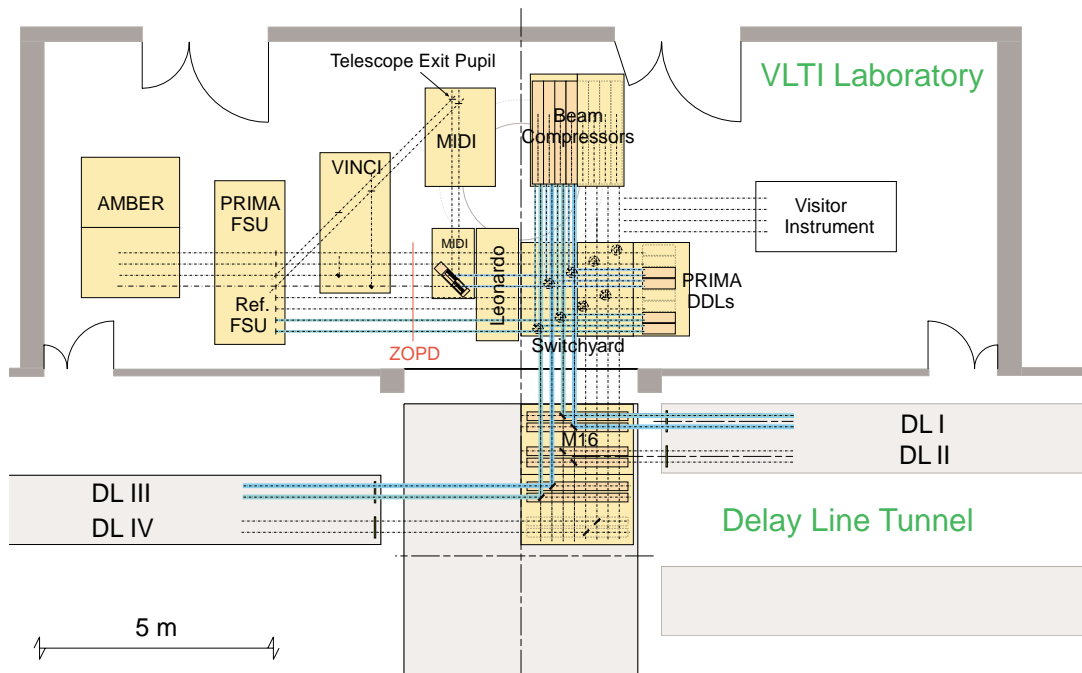
Figure 5. The layout of the VLTI Laboratory. The switchyard can direct the beam into four directions: 1) to the interferometric instruments (on the left) without beam compression, 2) to the interferometric instruments after beam compression, 3) to the Differential Delay Lines after beam compression, and 4) to the Differential Delay Lines without beam compression. The beam compressor reduces the beam diameter from 80mm to 18mm and it reimages the telescope pupil into the PRIMA FSU, MIDI and VINCI (the position of the pupil is indicated by a diagonal line). A possible location for a visitor instrument is shown on the right.
