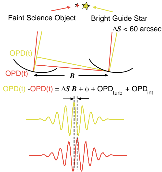
Figure 7. Principle of phase referenced imaging and astrometry with an interferometer. The difference in the positions of the white light fringes of object and reference star are determined by the OPD given by the product of \Delta S - the angular separation vector of the stars - and B - the baseline vector - by the phase \phi of the visibility function of the science object, by the OPD caused by the turbulence, and by the internal OPD.
