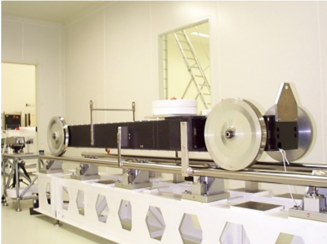
Figure 3. The carriage for the cat's-eye of the Delay Line System in the Clean Room at Fokker in Leiden. The carriage has three wheels running on the 65m steel rails. The diameter of the wheels is about 40cm and the length of the carriage 2.25m.
