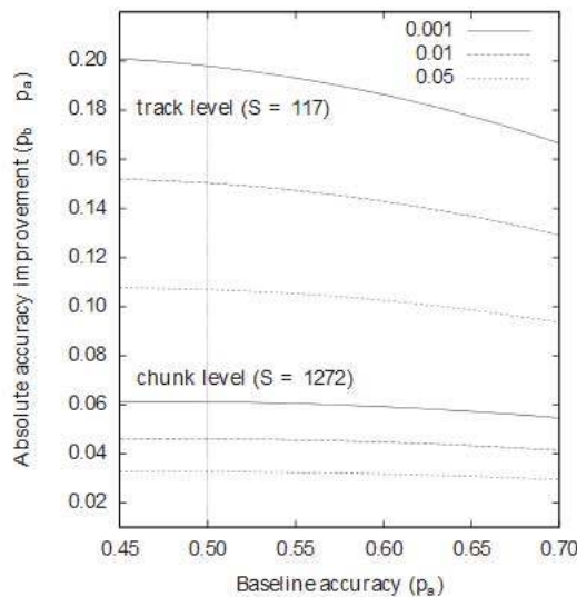
Fig. 3. Lines of significant absolute accuracy improvements for different levels of significance (0.001, 0.01, or 0.05), for experiments on the test set of the YouTube corpus, on track level (sample size S = 117 ) or chunk level ( S = 1272 ). Vertical line: chance level accuracy (0.5).
