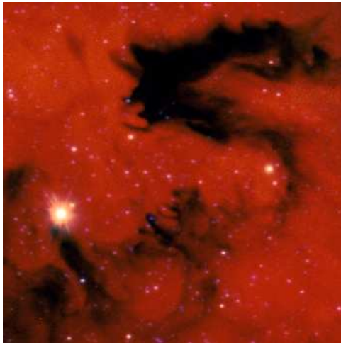
Figure 22. A cut-out at full resolution from M8, the Lagoon Nebula. This is an RGB image centred on RA 18 09 36 Dec - 24 01 51 (J2000), and spanning 150\times 150 arcsec 2 . The filters are combined such that R/G/B = H\alpha / i / r .
