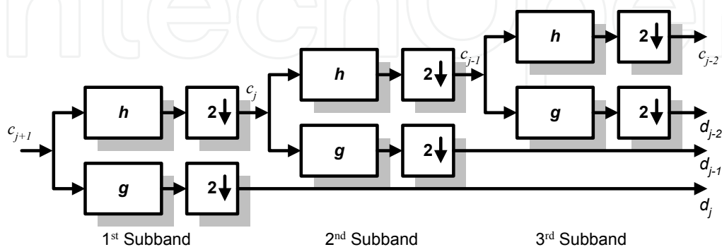
Fig. 7. Three-Stage analysis Subband Coding
