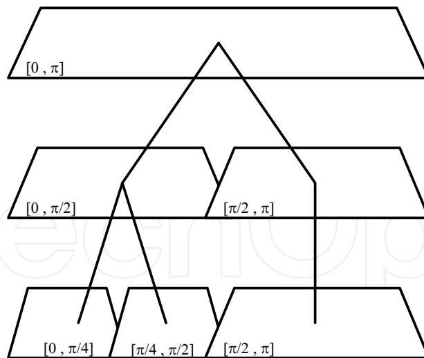
Fig. 15. Frequency bands of Feauveau's Quincux decomposition
