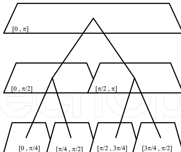
Fig. 13. Frequency Bands of Mallat's 2-D Analysis Algorithm
