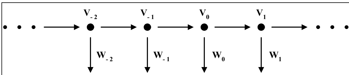
Fig. 4. Space decomposition
