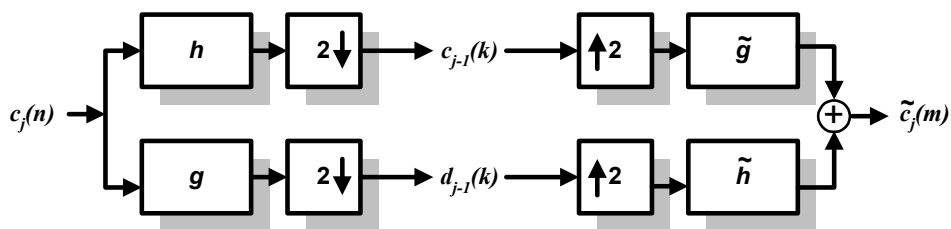
Fig. 18. Two-band analysis and synthesis filter bank
