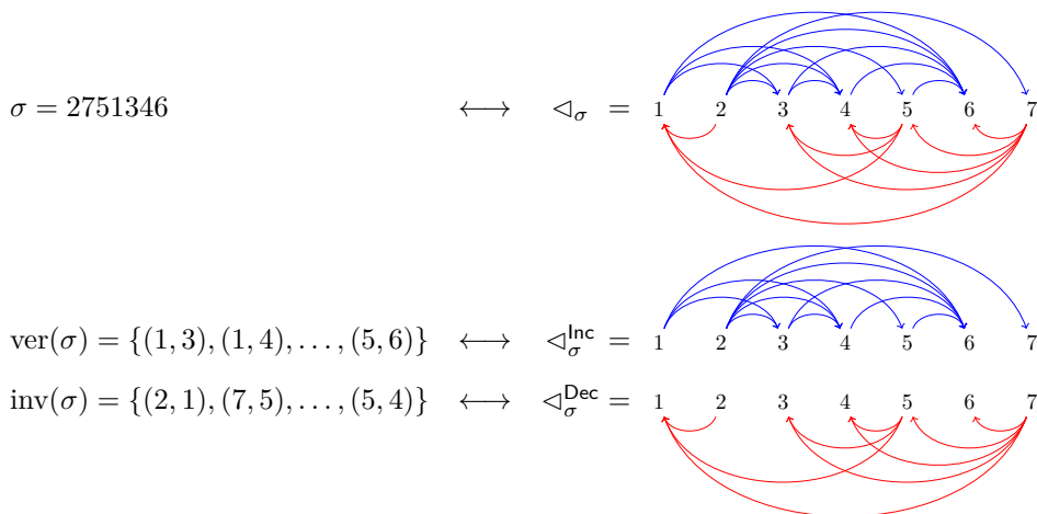
FIGURE 6. A Weak Order Element Poset (WOEP).
