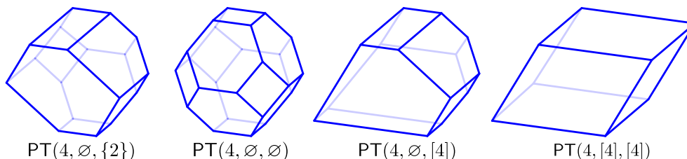
FIGURE 18. Four examples of permutreehedra. While the first is generic, the last three are a permutahedron, an associahedron [9], and a parallelepiped.
