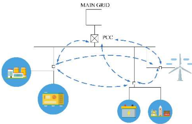
Figure 4. Decentralized adaptive scheme. Source: Authors
