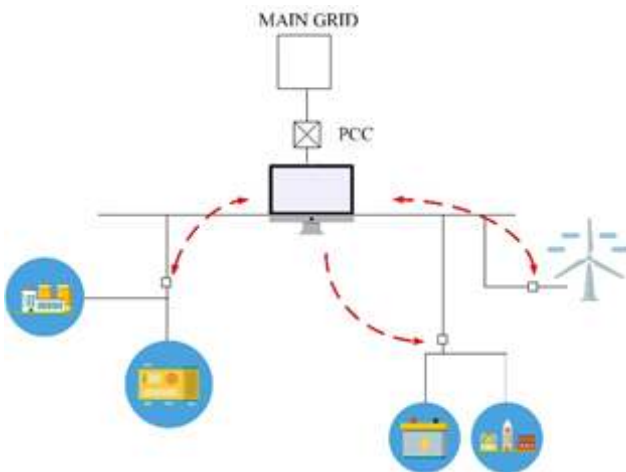
Figure 5. Centralized adaptive scheme. Source: Authors
