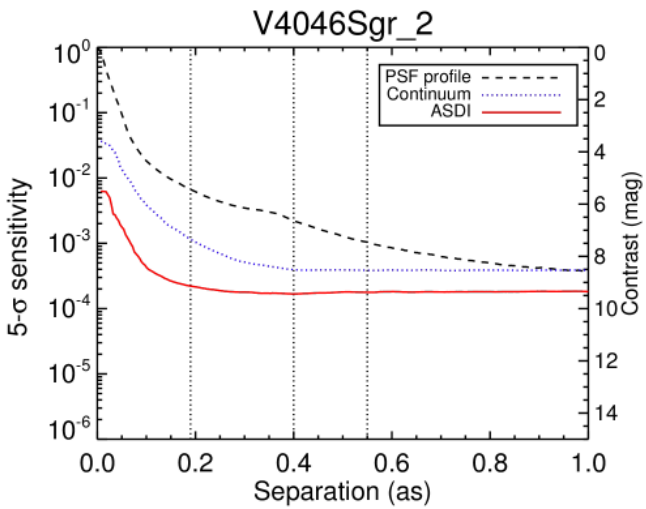
Fig. 4. Same as Fig. 3, but for the object V4046 Sgr. The vertical dotted lines represent the locations of the rings detected by Rapon et al. (2015) and Avenhaus et al. (2018).
