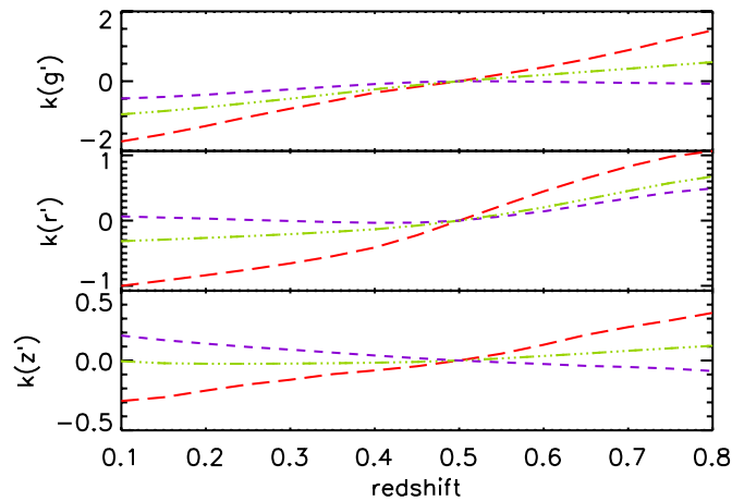
Figure 3. k -correction as a function of redshift for g'r'z' filters. The dashed red, dot-dashed green, and short-dashed purple curves are generated using the same model as in Figure 2, which represent evolved early-type red, mildly star-forming spiral, and star-forming late-type/irregular galaxies, respectively. (A color version of this figure is available in the online journal.)
