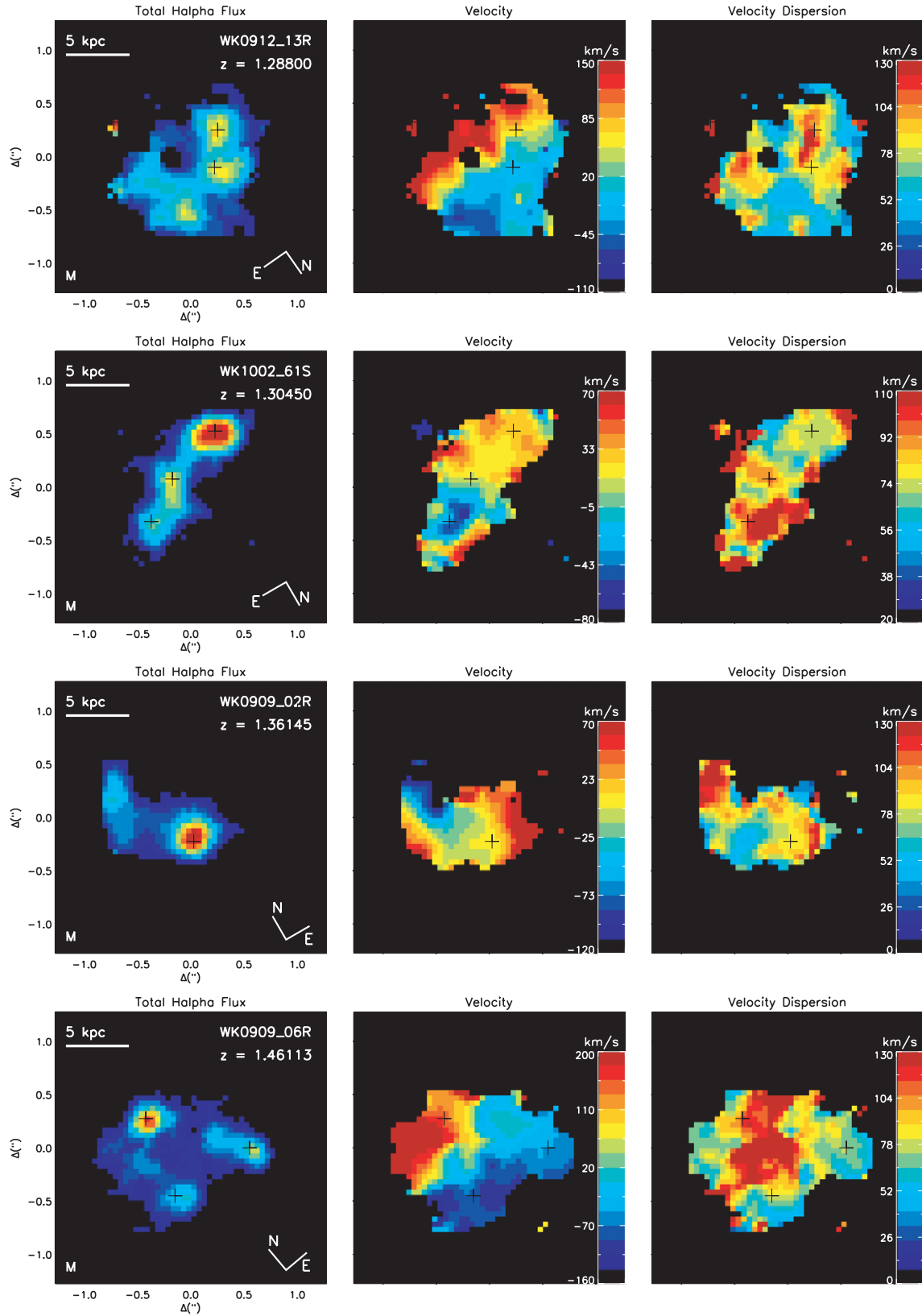
Figure 3. OSIRIS H\alpha kinematics. Left: H\alpha flux map; middle: velocity map from the systemic velocity; right: velocity dispersion map. The black crosses mark the peak(s) in H\alpha flux. Velocity shifts from the systemic redshift and velocity dispersion are measured in \text{km s}^{-1} . Compass at the bottom right of the left-hand panels shows the true orientation. Letters at the bottom left of the left-hand panels represent morphology classifications – M: multiple emission; E: extended emission; S: single emission. Objects are presented in the order based on the morphological classification described in Section 3.1.
