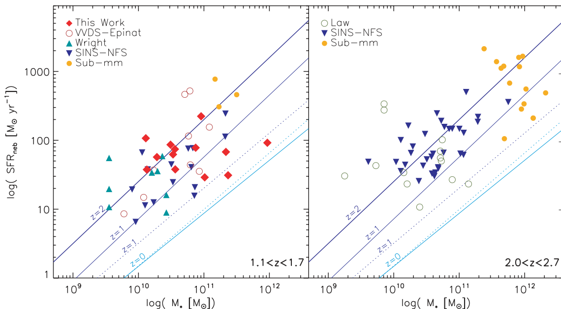
Figure 7. \text{H}\alpha SFRs of IFU samples at z > 1 as a function of stellar mass. Stellar masses and SFRs for all samples are converted to the Salpeter IMF for ease of comparison to the literature. The symbols are as described in Fig. 1. The solid lines are from the GOODS given in Elbaz et al. (2007) and Daddi et al. (2007). The dotted lines are from the Millennium Simulation (Springel et al. 2005; Croton et al. 2006) at redshifts z = 0 (light blue) and z = 1 (blue). An extinction correction is made from E(B - V)_{\text{SED}} .
