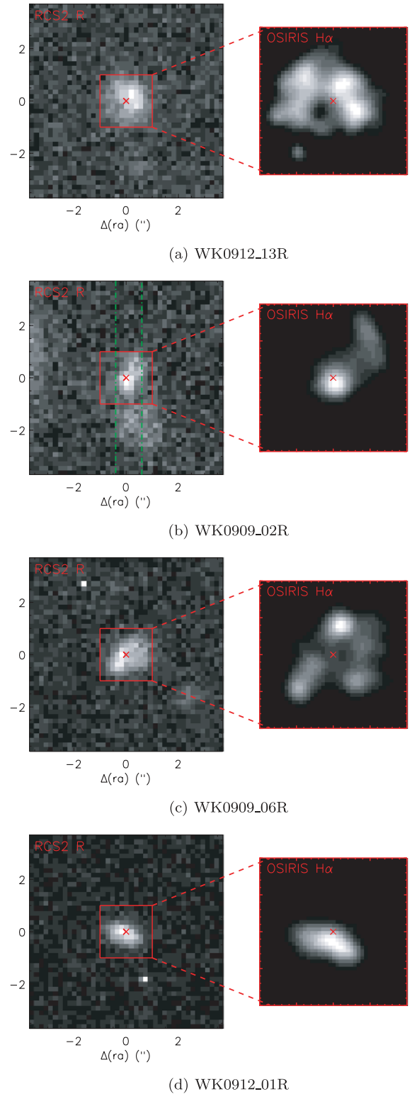
Figure A1. RCS2 r band and OSIRIS H \alpha images for 02R, 01R, 06R and 13R, the only objects with resolved broad-band imaging. The green dot-dash lines on the RCS2 image of 02R mark the position of the LRIS long slit. LRIS spectroscopy confirms the low surface brightness region below the central emission is at the same redshift as the central emission detected by OSIRIS.
