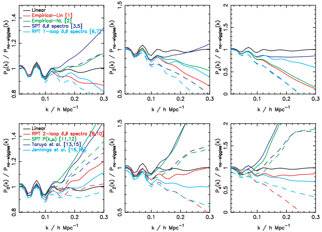
Figure 4. The multipole power spectra P_\ell(k) for \ell = 0, 2, 4 for the different models listed in Table 1. The models are evaluated at redshift z = 0.6 assuming a linear bias b = 1 , a growth rate f = 0.7 and (where applicable) a damping term \sigma_v = 300 h \text{ km s}^{-1} . The models are labelled by their row number in Table 1. The solid and dashed lines are models that, respectively, include and exclude the damping term. All models are divided by a smooth ‘no-wiggles’ reference power spectrum from the fitting formulae of Eisenstein & Hu (1998), which has the same shape as the linear power spectrum but without the imprint of baryon acoustic oscillations. The models agree well in the large-scale limit, but significant differences develop between the models at smaller scales.
