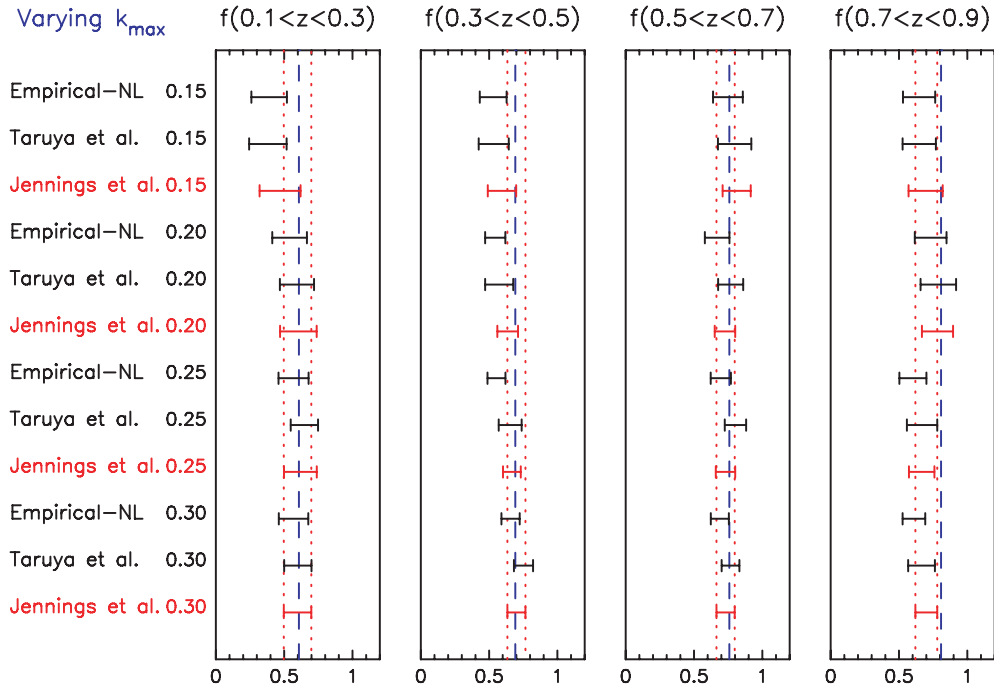
Figure 7. Measurements of the growth rate f in four redshift slices, varying the fitting limit k_{\max} from 0.15 to 0.30 h \text{ Mpc}^{-1} in steps of 0.05, for the three optimal models: the non-linear empirical Lorentzian, Taruya et al. (2010) and Jennings et al. (2011) models. All models include a variable damping parameter. The vertical dashed line indicates the prediction of a flat \Lambda CDM cosmological model with \Omega_m = 0.27 . The two vertical dotted lines span the 68 per cent confidence region of the growth rate measured for the Jennings et al. model for k_{\max} = 0.3 , facilitating an easy comparison of the results for different models.
