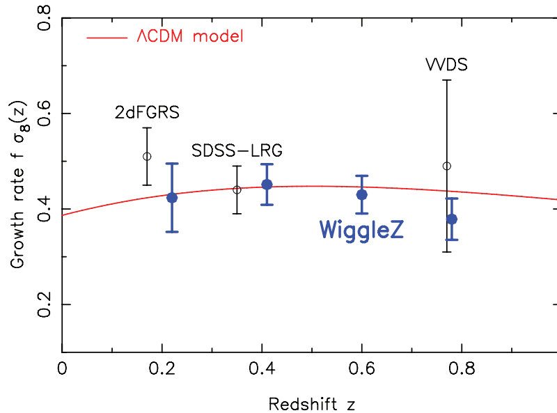
Figure 8. Measurements of the growth rate of structure weighted by a redshift-dependent normalization, f(z)\sigma_g(z) , obtained in four redshift slices by fitting WiggleZ Survey data. We assume the Jennings et al. (2011) model for non-linear redshift-space distortions, with a variable damping parameter, and fit to the scale range k < 0.3 h\text{Mpc}^{-1} . The WiggleZ measurements are compared to results previously published for the 2dFGRS, SDSS-LRG and WVDs samples (black open circles) as collected by Song & Percival (2009). The prediction of a flat \Lambda\text{CDM} cosmological model with \Omega_m = 0.27 is also shown.
