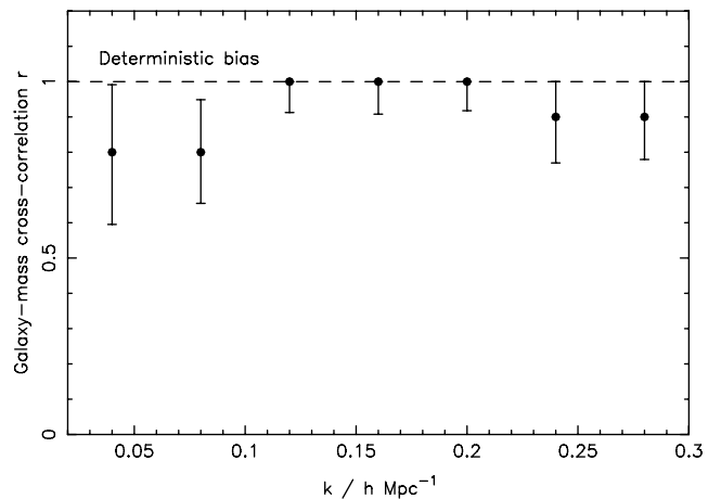
Figure 9. The galaxy–mass cross-correlation parameter r as a function of scale k , measured by fitting equation (14) to the WiggleZ power-spectrum data assuming the growth rate predicted by \Lambda\text{CDM} and marginalizing over a linear bias and variable damping factors. The measurements in different redshift slices are combined.
