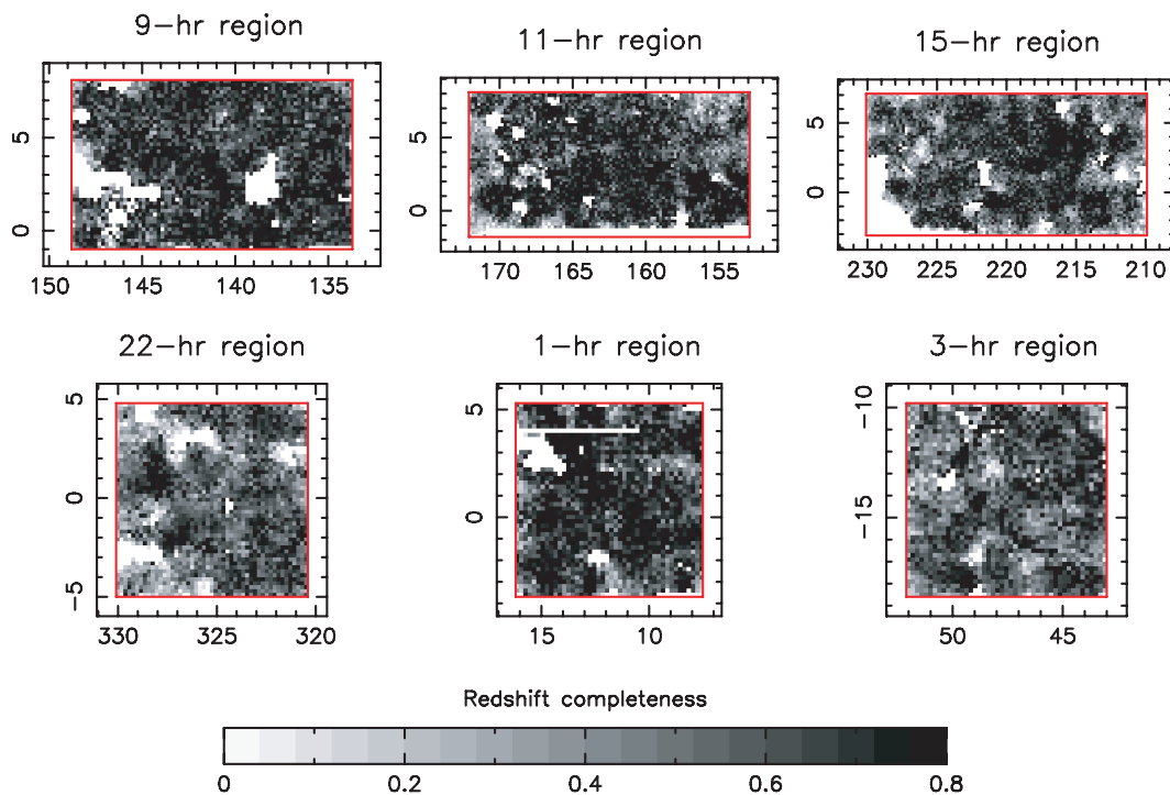
Figure 1. Grey-scale map illustrating the relative redshift completeness of each of the six WiggleZ Survey regions analysed in this paper. This figure is generated by taking the ratio of the galaxy densities in the redshift and parent catalogues in small cells. The x - and y -axes of each panel represent right ascension and declination, respectively.
