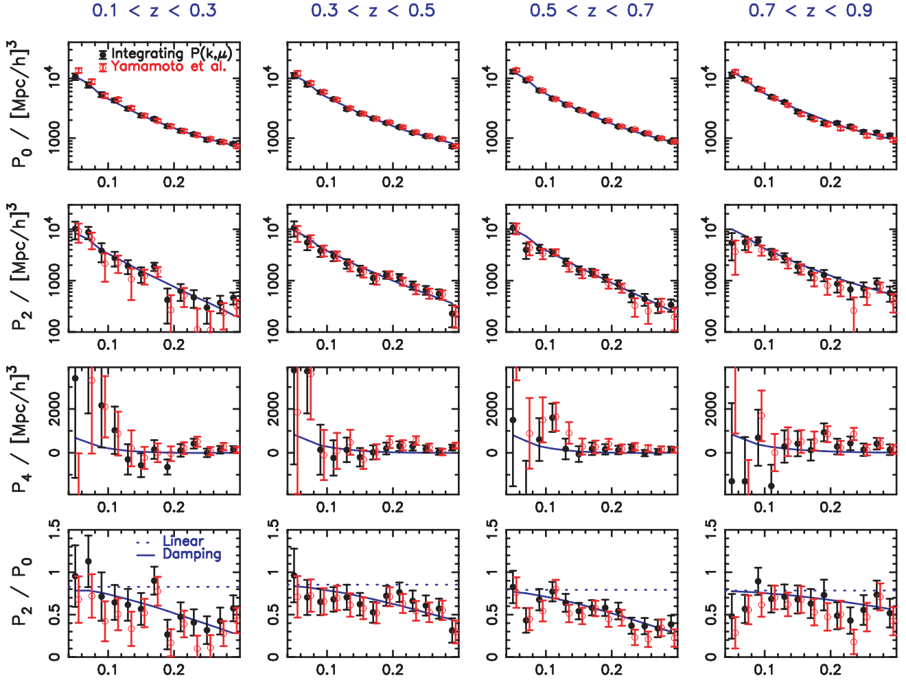
Figure 10. The multipole power spectra P_\ell(k) for \ell = 0, 2, 4 for WiggleZ Survey observations in four redshift slices. The monopole ( \ell = 0 ) spectrum primarily contains information about the underlying shape of the isotropic clustering pattern. The quadrupole ( \ell = 2 ) spectrum holds the leading-order signal from the anisotropic modulation in power due to redshift-space effects. The (black) solid circles are generated from the stacked measurements of P_g(k, \mu) across the different survey regions using equation (17). The (red) open circles, which are offset slightly in the x -direction for clarity, are generated by combining the estimates of P_\ell(k) in each region using the Yamamoto et al. estimator of equation (19). The model lines correspond to the best-fitting non-linear empirical Lorentzian redshift-space distortion model in each case. The bottom row displays the quadrupole-to-monopole ratio P_2(k)/P_0(k) . Two models are overplotted: the large-scale Kaiser limit predicted in a \Lambda CDM cosmological model with \Omega_m = 0.27 , labelled as ‘linear’, and the non-linear redshift-space distortion model, labelled as ‘damping’.
