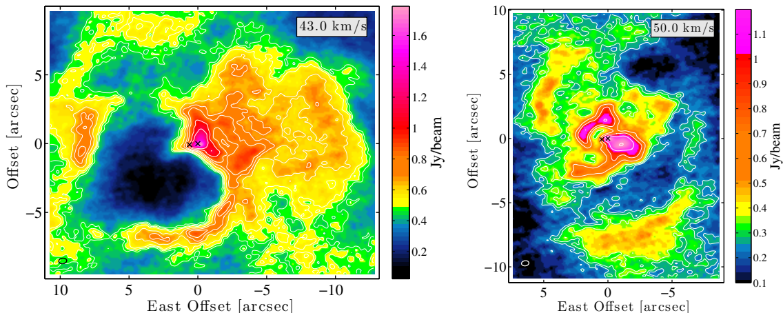
Fig. 3. CO(3–2) map averaged over 2 and 3 \text{km s}^{-1} around v_{\text{lsr}} = 43.0 and 50.0 \text{ km s}^{-1} , respectively, showing the bubble structure ( left ) and the spiral arcs ( right ) discussed in Sect. 3.2. The crosses mark the position of Mira A (west) and B (east). Contours are drawn at multiples of the rms noise level. The beam is shown in the lower left corner.
