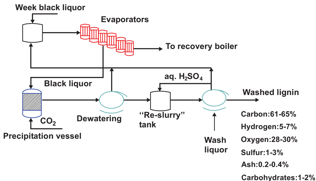
Fig. (3). The LignoBoost process and composition of the obtained kraft lignin [3].
