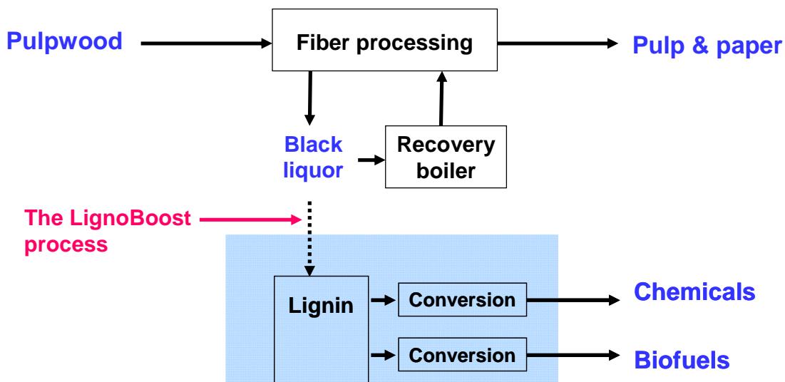
Fig. (2). A future kraft pulp mill with partial withdrawal of lignin according to the LignoBoost process [3].
