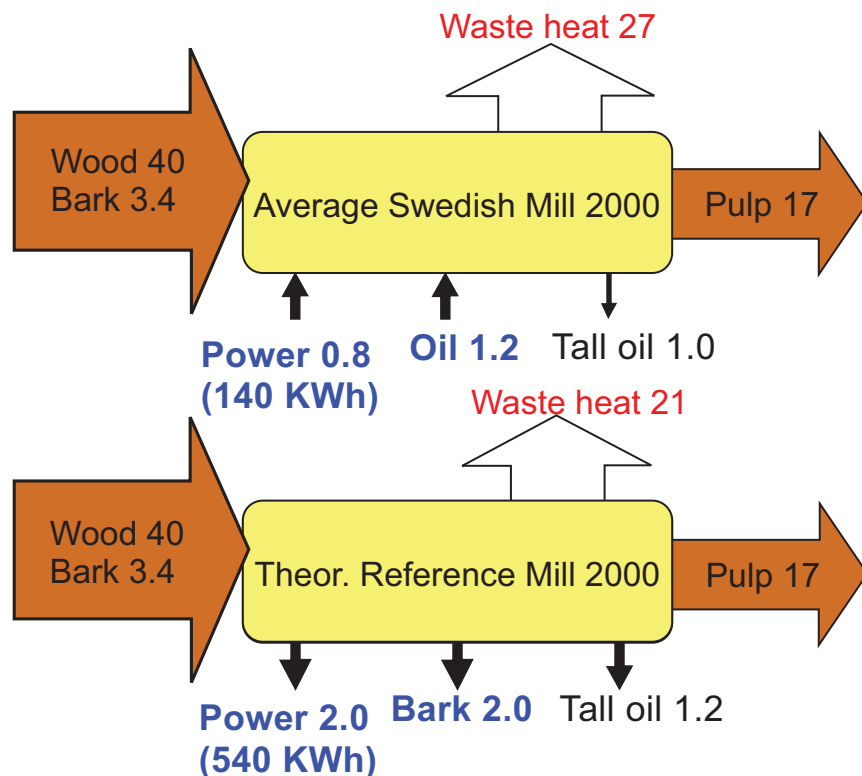
Fig. (1). Energy balance in kraft pulp mills expressed in GJ/ton of pulp; the Swedish average mill in 2000 and a theoretical reference mill equipped with state-of-the-art technology in 2000 [2].
