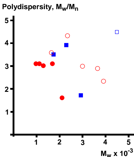
Fig. (4). Polydispersity of softwood (squares) and hardwood (circles) kraft lignins before (unfilled) and after purification (filled) by either solvent or membrane fractionation. Data from [20, 23-25].
