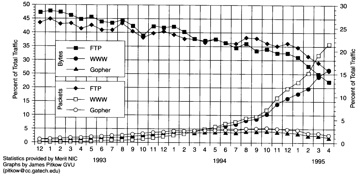
FIG. 1. Merit NIC Backbone statistics for the Web, Gopher and FTP from 1993–1995 in terms of both packet and byte counts (source: Merit NIC and Jim Pitkow [18], used with permission).
