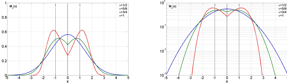
Figure 2: Plots of the symmetric M -Wright function with \nu = 1/2, 5/8, 3/4, 1 for -5 \leq x \leq 5 ; left: linear scale; right: logarithmic scale.
