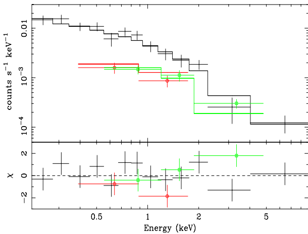
Fig. 3. EPIC spectrum of the X-ray afterglow of GRB 030329 fitted with a power law model. Upper line and data refer to the PN, lower ones to the MOS. The bottom panel shows the best fit residuals in units of standard deviations.
