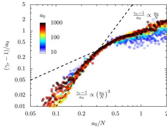
Figure 10. Peak Lorentz factor in the direction of emission for the emitting electron bunch for varied a_0 and N at \theta_L = 30^\circ . Since \gamma - 1 \propto a_0 , the normalized quantity (\gamma^{\max} - 1)/a_0 collapses to a single curve f(a_0/N) asymptotically for a_0 \rightarrow \infty , with two distinct power-law regimes. For low a_0/N , the Lorentz factor approximately scales with (a_0/N)^3 and for a_0/N > 0.3 , corresponding to the initial onset of the relativistic transparency regime, it scales proportional to a_0/N . Each point is extracted from a separate PIC simulation with a single-cycle driving laser.
