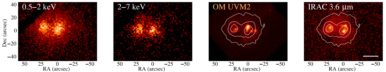
Fig. 2. XMM-Newton /EPIC pn 0.5–2 keV and 2–7 keV images (first and second panels), XMM-Newton /OM UUVW2 (2120 Å) images for the galaxies observed with this filter (third panel). The third panel of Arp299 and MCG+04-48-002 corresponds to the XMM-Newton /OM UVM2 (2310 Å) filter. Spitzer /IRAC 3.6 μm images (fourth panel). For reference we represent in the third and fourth panels the smoothed 0.5–7 keV contours. The white line in the right panels represents 5 kpc at the distance of the galaxy. All images are shown in a square root scale. North is up and east is to the left.
