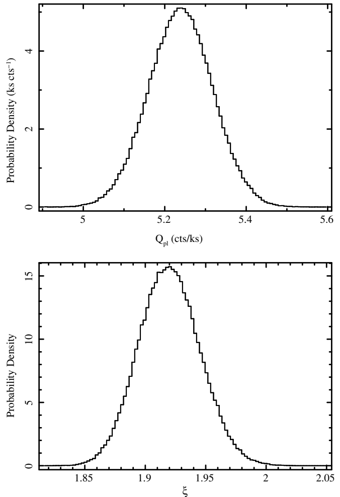
Figure 3. MCMC PDFs for the quiescent rate Q_{pl} (top) and the power-law index \xi (bottom) marginalized over \xi and Q_{pl} , respectively. Both distributions are well behaved. Note that as probability densities, these curves integrate to 1.
