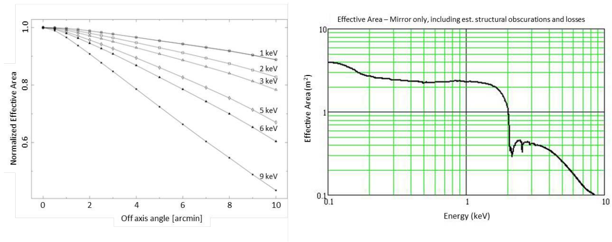
Figure 3. (Left) Vignetting as a function of energy and field. (Right) On-axis effective area prediction for X-ray Surveyor . The area at 1 keV is 2.3 \text{ m}^2 . This calculated effective area includes structural obscuration, misalignments, particulate contamination and scatter. This is roughly 30x that of the Chandra High Resolution Mirror Assembly (HRMA).
