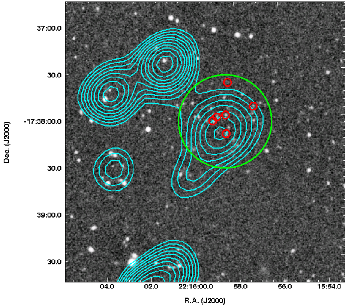
Fig. 1.— K_s -band image of a 3 arcmin field centered on the cluster with an X-ray overlay of contours in blue. The 6 spectroscopically confirmed members are circled in red (ID=14651 is not detected in the K_s image). The green circle of diameter 60 arcsec shows the location of the region used for the X-ray analysis reported in section 3.1.
