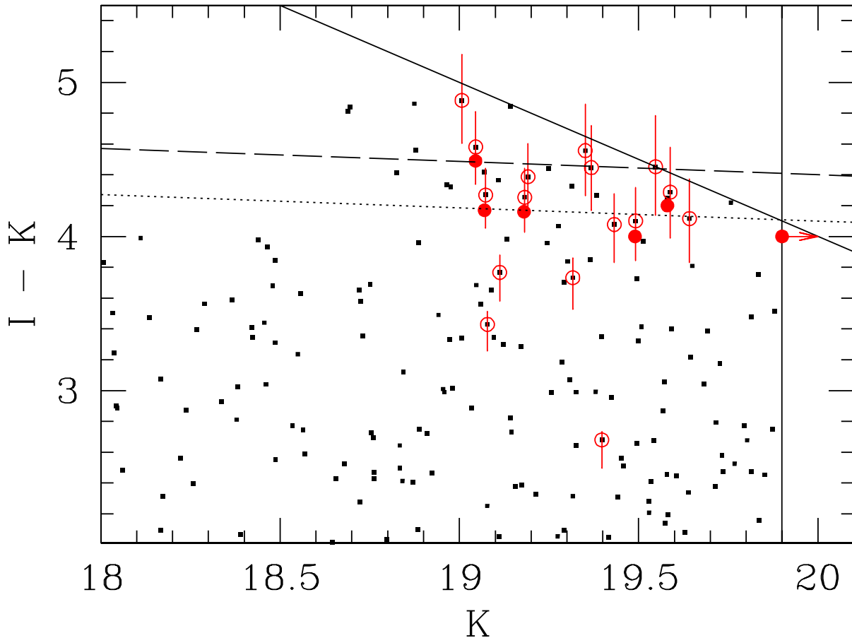
Fig. 2.— An I - K_s vs K_s color-magnitude diagram for XMMXCS J2215.9-1738; aperture magnitudes are used for the colors and K_s magnitudes. The black points are all the objects within a 3 arcmin box around the position of the X-ray source, and the objects circled in red lie within 30 arcsec of the center of the X-ray source. The solid red points are those with concurrent spectroscopic redshifts at z = 1.45 . The dashed (dotted) line represents the expected color-magnitude relation for galaxies as predicted by a Bruzual & Charlot model in which all the stars formed within a 0.1 Gyr burst starting at z_f = 3 ( z_f = 2 ) in the standard cosmology. The solid lines represent the 5\sigma limits to the K_s and I - K_s photometry.
