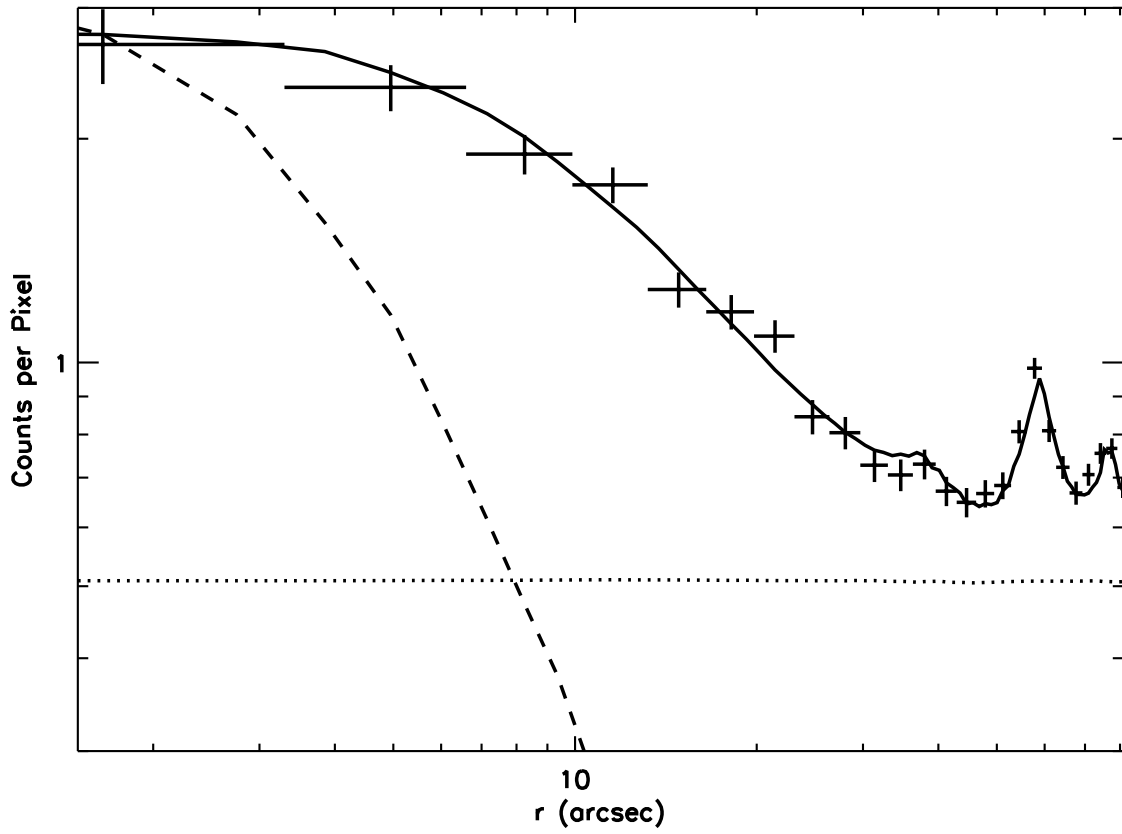
Fig. 3.— The spatial profile of the X-ray emission. The points are the data. The best fitting model, combining both the extended component and the point sources (which are obvious as bumps at large radii), is shown by the solid line. A PSF is shown by the dashed line. The background is shown by the horizontal dotted line.
