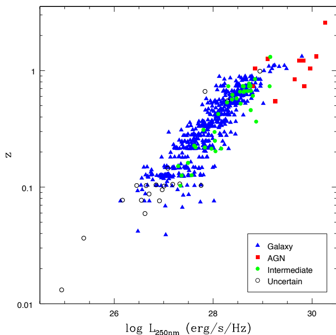
Fig. 9. L_{250nm} - z plane for the extragalactic objects. Symbols and colours are defined as in Figure 3 and reported in the legend.
