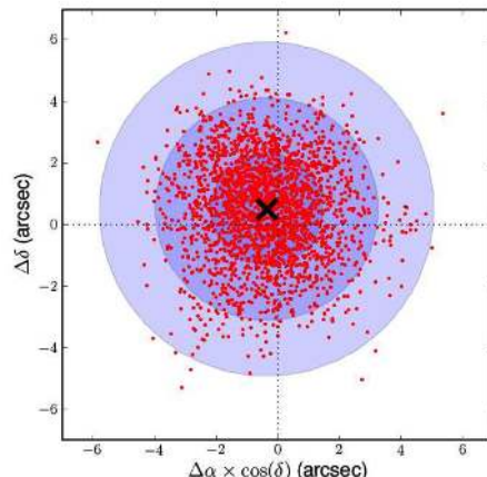
Figure 4. Using source correlations between the XMM-OM source tables and the USNO-B1.0 catalog, systematic corrections are applied to the recorded XMM-OM pointings and source positions. The above plot summarizes the full sample of pointing offsets applied in both the RA ( \alpha ) and Dec ( \delta ) directions (red dots). The black cross is the mean correction and the blue circles represent 1-, 2- and 3- \sigma deviations from the mean.
