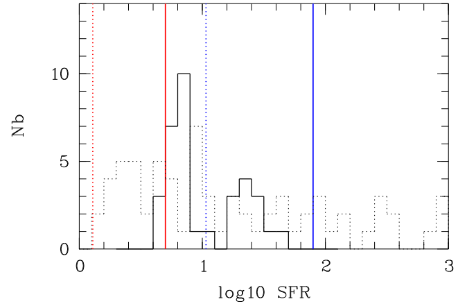
Fig. 7. Comparison of our stellar mass and SFR estimates for the XLSSC 116 ICL source (red vertical line for SED estimation and red vertical dotted line for spectroscopic estimation) and BCG (blue vertical line for SED estimation and blue vertical dotted line for spectroscopic estimation) with the Puech et al. (2010) emission line galaxies (continuous histograms) and the Liu et al. (2012) BCGs (dashed histograms). Upper figure: stellar mass, lower figure: SFR.
