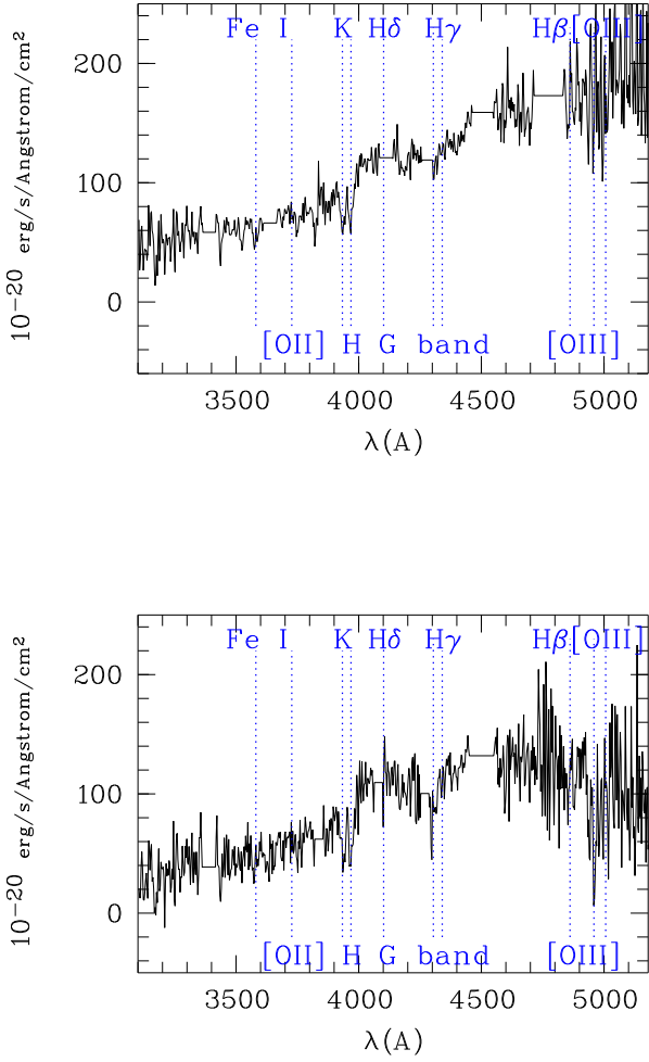
Fig. 8. Mean (upper figure) and median (lower figure) rest frame spectrum of all the galaxies spectroscopically measured inside the cluster (excluding the BCG). Strong sky lines have been masked. The position of the most common lines are shown as dashed lines.
