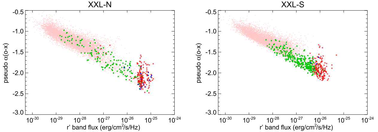
Fig. 8. Proxy for the \alpha_{ox} index for XXL-N ( left panel ) and XXL-S ( right panel ) as a function of optical flux. The optical-to-X-ray spectral index is defined as \alpha_{ox} = \log(f_x/f_o)/\log(\nu_x/\nu_o) where the optical monochromatic flux is computed from the r' AB magnitude 2.5\log f_o = -r' - 48.6 , and the reference frequency \nu_o derived from the \lambda_{\text{eff}} of the filter (6258Å for CFHT, 6185Å for SDSS, 6266Å for BCS, and 6433Å for DECam); \nu_x corresponds to 2 keV; the monochromatic 2 keV flux f_x is extrapolated from the observed [0.5–2 keV] soft flux F_{\text{soft}} using the spectral model of Table 2, i.e. f_x = 7.626176 \times 10^{-27} \times 2 \times 1.47115 \times 10^8 F_{\text{soft}} . Only sources detected in the soft X-ray band with a primary counterpart in the r' filter are considered. Symbols and colour-codes are as in Fig. 7.
