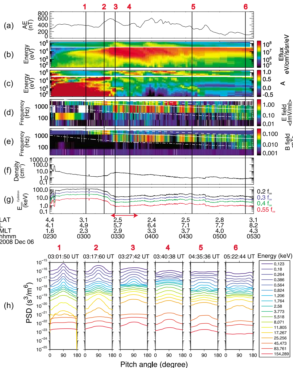
Figure 7. (a) AE index and ((b) and (c)) the time evolution of the omnidirectional electron energy flux ( \text{eV}/\text{cm}^2/\text{s}/\text{sr}/\text{eV} ) and anisotropy for various energies (100 eV–200 keV) from 0230 to 0530 UT on 6 December 2008 observed by Time History of Events and Macroscale Interactions During Substorms (THEMIS) D. (d) and (e) Amplitudes of wave electric and magnetic fields from the filter bank data given in units of mV/m and nT, respectively. The three white lines represent the equatorial electron cyclotron frequency ( f_{ce} ) (dashed), 0.5 f_{ce} (solid), and 0.1 f_{ce} (dash-dotted). (f) Total plasma density ( \text{cm}^{-3} ) inferred from the spacecraft potential. (g) Minimum electron energy for cyclotron resonance with chorus waves of various frequencies (black: 0.2 f_{ce} , blue: 0.3 f_{ce} , green: 0.4 f_{ce} , and red: 0.55 f_{ce} ). The horizontal red arrow indicates the time period when particle burst data are available. (h) Six vertical black arrows represent six snapshots, which show the time evolution of the electron PSD as a function of the pitch angle for 18 different energy levels (0.123–154.289 keV).
