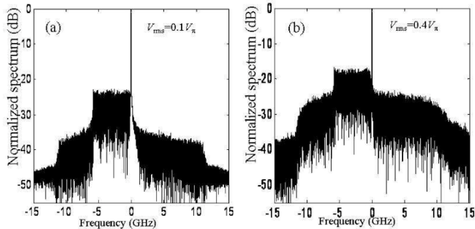
Fig. 3. Optical spectra of compatible-SSB OFDM signal with small modulation index (a) and large modulation index (b).
