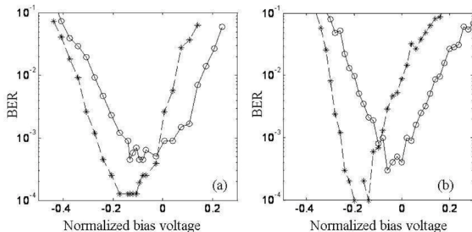
Fig. 6. BER versus normalized bias voltage variation from the quadrature point for back-to-back (stars) and over three fiber spans (open circles). (a) measured and (b) numerical simulation
