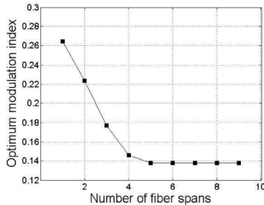
Fig. 8. Simulated optimum modulation index as the function of fiber length. Modulation index is defined as the rms driving signal voltage divided by V_{\pi} .
