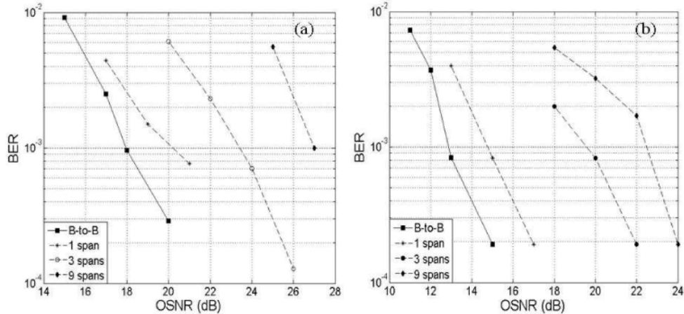
Fig. 9. BER versus OSNR for different transmission distances. (a) measured and (b) numerical simulation
