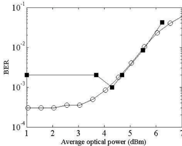
Fig. 11. Measured (solid squares) and simulated (open circles) BER versus launch power for compatible-SSB OFDM system after 675km fiber transmission
