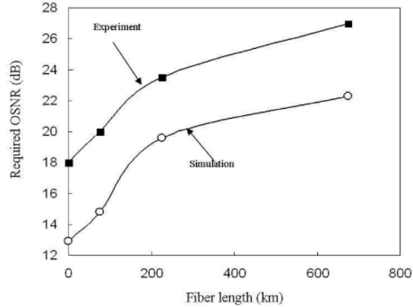
Fig. 10. Required OSNR versus fiber length.
