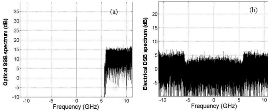
Fig. 1. Spectra of offset-SSB modulation (a) optical single-sideband spectrum, and (b) electrical double-sideband spectrum after square law detection
