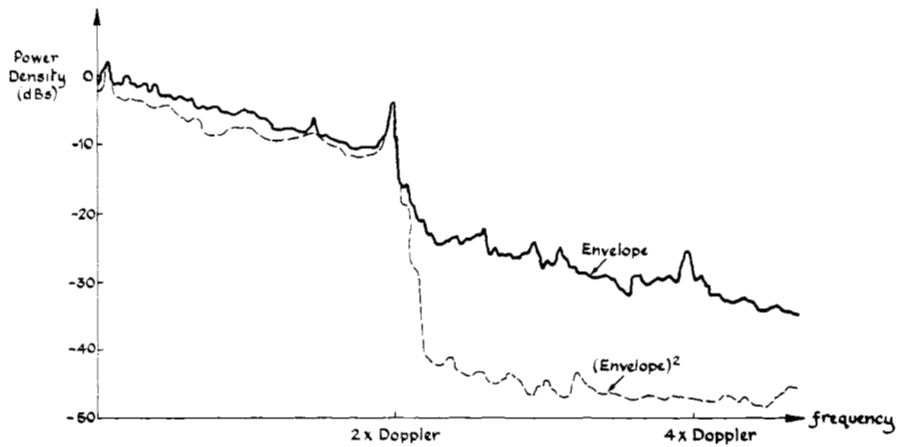
Fig. 12. Power density spectra of fading pilot tone envelope and (envelope) 2 .
