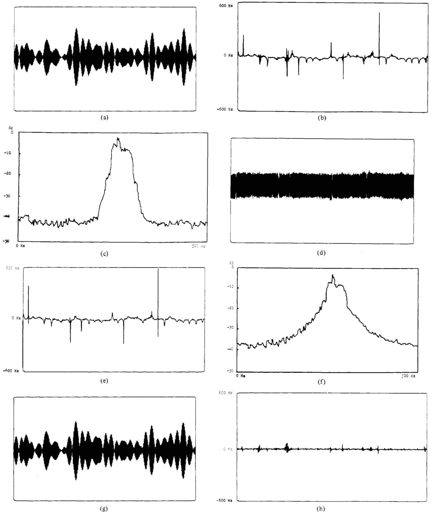
Fig. 11. (a) Envelope variation (FFSR circuit input). (b) Instantaneous frequency deviation (FFSR circuit input). (c) Power density spectrum (FFSR circuit input). (d) Envelope variations (FFAGC output). (e) Instantaneous frequency deviation (FFAGC output). (f) Power density spectrum (FFAGC output). (g) Envelope variation (FFAFC output). (h) Instantaneous frequency deviation (FFAFC output). (i) Power density spectrum (FFAFC output). (j) Envelope variation (FFSR output). (k) Instantaneous frequency deviation (FFSR output). (l) Power density spectrum (FFSR output).
