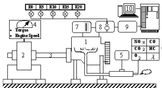
Figure 1. Schematic diagram of experimental setup. 1-Engine, 2-Dynamometer, 3- Drive shaft, 4- Dynamometer control unit, load and speed indicator, 5- Temperature indicator, 6- Gas
