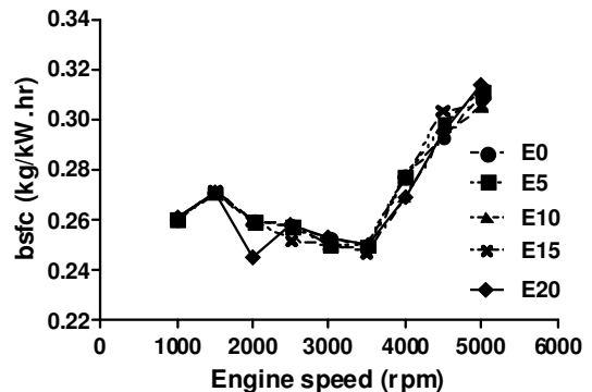
Figure 6. Experimental results of brake specific fuel consumption at different fuel blends and engine speeds
