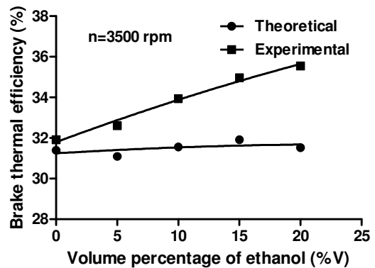
Figure 14. brake thermal efficiency with volume percentage of ethanol at WOT condition
