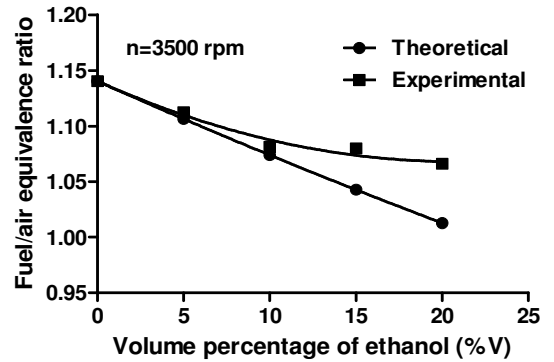
Figure 11. Fuel/air equivalence ratio with volume percentage of Ethanol at WOT condition
