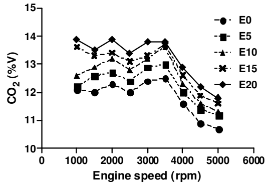
Figure 8. Experimental results of CO 2 at different gasoline-ethanol blends and engine speeds
