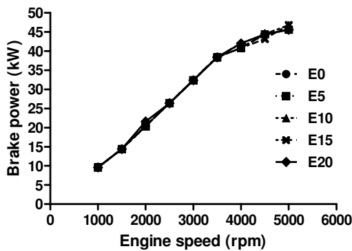
Figure 2. Experimental results of brake power at different fuel blends and engine speeds
