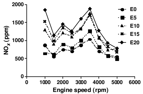
Figure 10. Experimental results of NO x at different gasoline-ethanol blends and engine speeds
