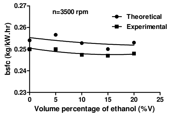
Figure 15. brake specific fuel consumption with volume percentage of ethanol at WOT condition
