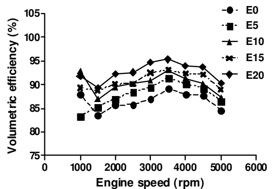
Figure 5. Experimental results of volumetric efficiency, at different fuel blends and engine speeds
