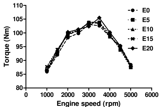
Figure 3. Experimental results of Torque, at different fuel blends and engine speeds
