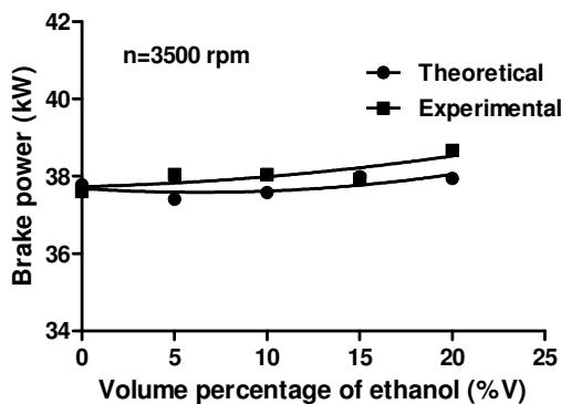
Figure 13. brake power with volume percentage of ethanol at WOT condition
