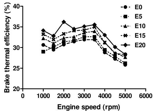
Figure 4. Experimental results of brake thermal efficiency, at different fuel blends and engine speeds
