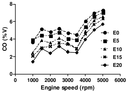
Figure 7. Experimental results of CO at different gasoline-ethanol blends and engine speeds
