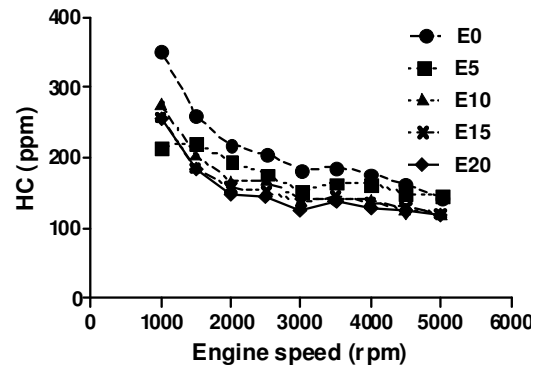
Figure 9. Experimental results of HC at different gasoline-ethanol blends and engine speeds
