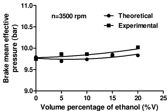
Figure 12. brake mean effective pressure with volume percentage of ethanol at WOT condition
