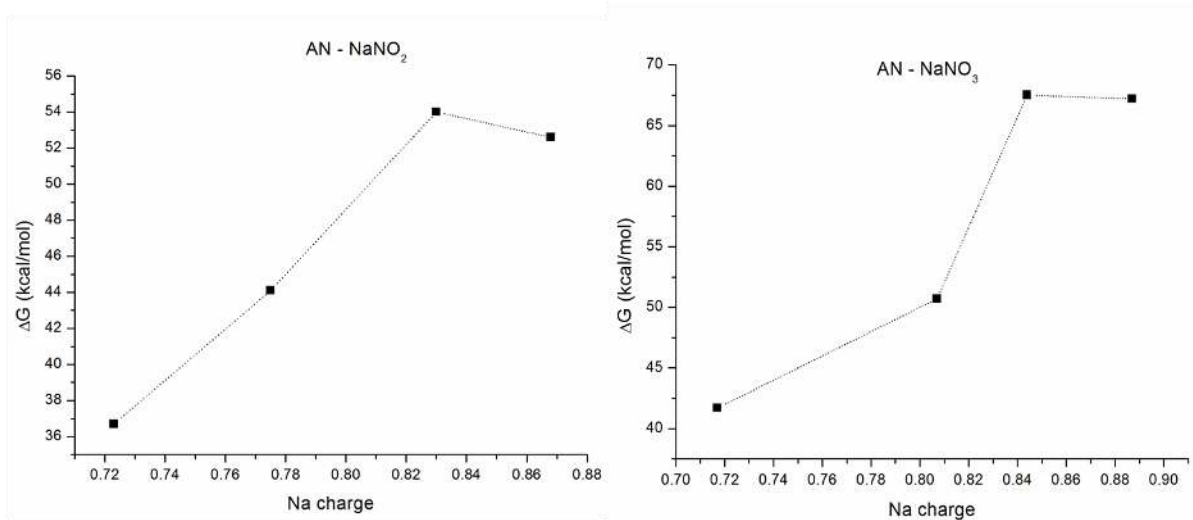
Figure 4. Relation between the Mulliken sodium charge and the activation energy for the reaction AN + NaNO 2 and AN + NaNO 3 with a water molecule.
