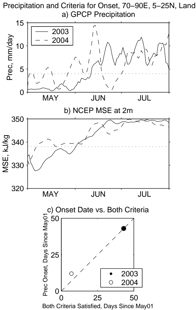
Fig. 23. Precipitation onset date vs. moist static energy and vertical velocity criteria for the onset in observation-based data over the region 70^{\circ} – 90^{\circ} E, 5^{\circ} – 25^{\circ} N (land part) during 2003 and 2004 (all-India onset was substantially delayed in 2003 as compared to 2004.) (a) time series of GPCP (Huffman et al., 2001) precipitation. (b) time series of moist static energy at 2 m. (c) onset date vs. the day when both the criteria were satisfied.
