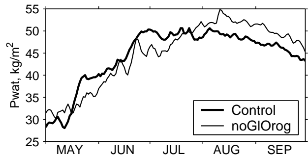
Fig. 7. Evolution of P wat (kg m -2 ) over the Indian region in control and noGIOrag simulations.
