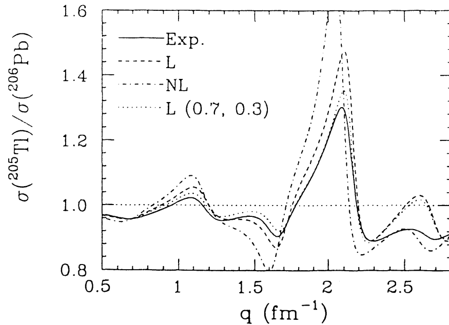
Fig. 2. Cross section ratio for ^{206}\text{Pb} - ^{204}\text{Hg} . The curves are as described in figure 1.
