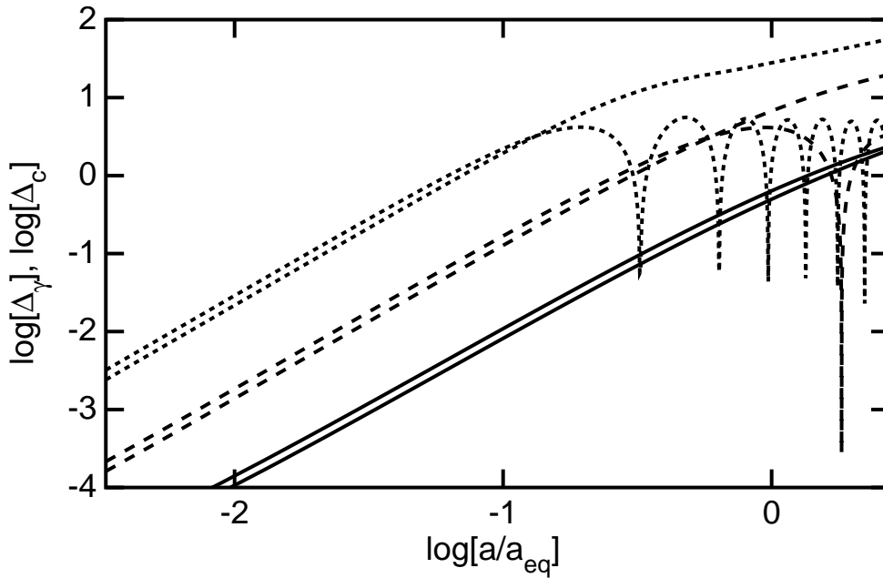
Fig. 1.6. Density contrasts in the CDM and the photons for wavenumbers \kappa = 5, 20, and 80 (see Fig. 1.7) as a function of the scale factor relative to the scale factor and when matter and radiation densities were equal. The photon density contrast starts out slightly larger than the CDM density contrast but oscillates.
