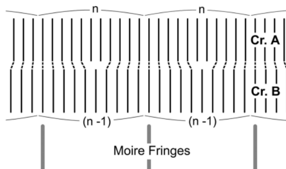
Figure 4 Schematic illustration to explain the generation of moiré fringes based on equation (37c) with \Delta\rho = 0 .
