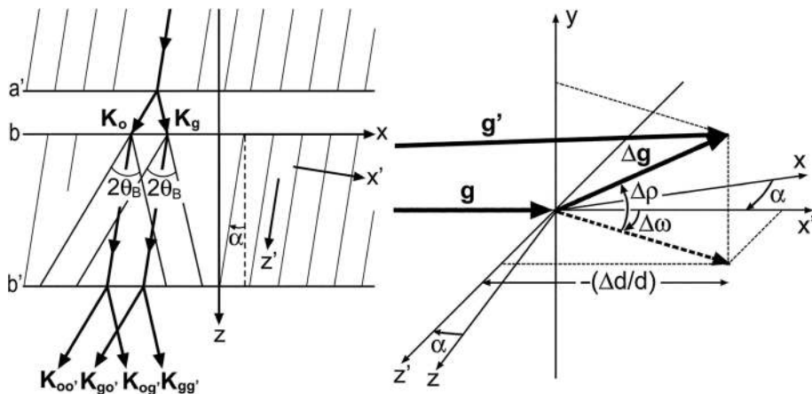
Figure 3 Coordinate systems in the discussion of the moiré phase, and graphical representation of components of \Delta\mathbf{g} . The two triangles in the left-hand side figure represent Borrmann fans for the incidence of the waves, \mathbf{K}_o and \mathbf{K}_g . In this diagram \hat{\mathbf{K}}_o = [-\sin(\theta_B + \alpha), 0, \cos(\theta_B + \alpha)] and \hat{\mathbf{K}}_g = [\sin(\theta_B - \alpha), 0, \cos(\theta_B - \alpha)] .
