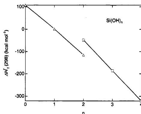
Figure 2. Calculated heats of formation for Si(OH) n species as a function of n . Triangles: species on this line (Si 3 P, SiOH( 2 A''), and Si(OH) 2 (singlet), have an s 2 p 2 electronic configuration at Si, causing their heats of formation to fall along a straight line. Squares: species on this line (Si(OH) 2 (triplet), Si(OH) 3 , and Si(OH) 4 ) have an sp 3 electronic configuration at Si, causing their heats of formation to fall along a different line.
