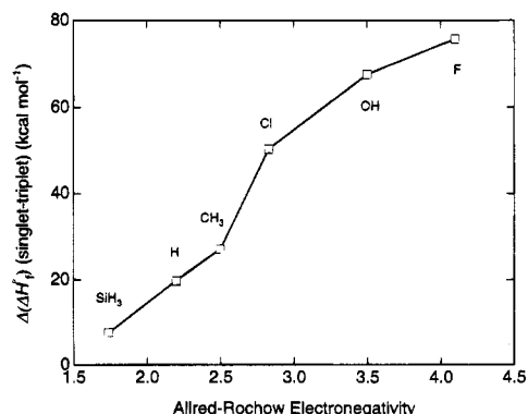
Figure 3. Singlet–triplet splittings for SiR 2 species as a function of the Allred–Rochow electronegativity. The identity of R is shown on the figure.
