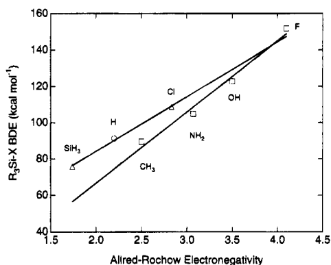
Figure 4. Si–X bond dissociation energies for R 3 SiX compounds as a function of the Allred–Rochow electronegativity. Triangles indicate BDEs for second-row X groups, hydrogen is indicated by a circle, and squares indicate BDEs for first-row X groups. Lines shown are linear least-squares fits to each set.
