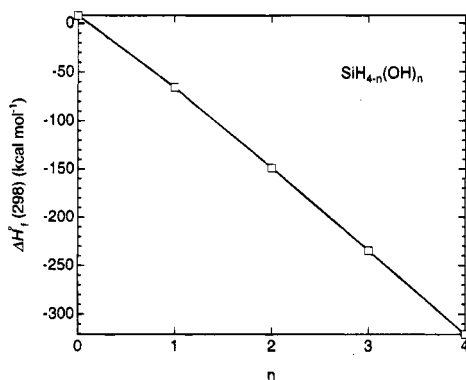
Figure 1. Calculated heats of formation for SiH 4-n (OH) n species as a function of n . As expected for closed-shell molecules, these species fall nearly on a straight line.
