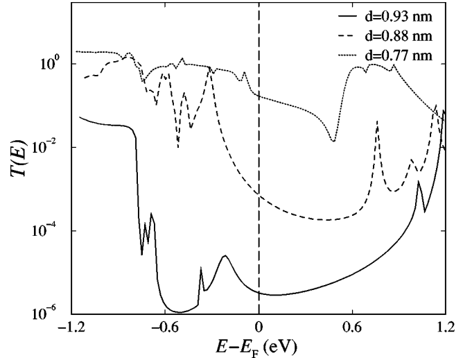
FIG. 2. Transmission spectra for the relaxed configuration with orientation (5) (see Fig. 1) for different distances d between the nanotubes.
