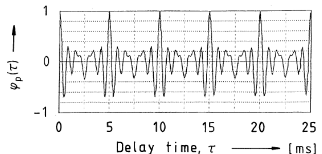
Fig. 6. Normalized autocorrelation function (NACF) of the two complex tones with its period of 5 ms (200 Hz).
