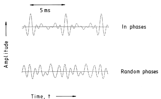
Fig. 5. Real waveforms of the complex tone in phase components (above) and in random phase components (below).
