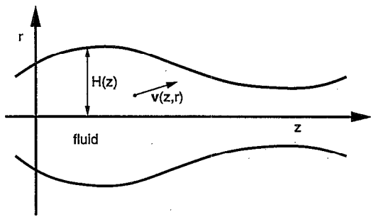
FIG. 1. A sketch of the flow geometry investigated in the present paper. The radius or "height" of the free surface at a point z on the axis of symmetry is H(z) . The velocity field inside the fluid is \mathbf{v}(z,r) = v_z(z,r)\mathbf{e}_z + v_r(z,r)\mathbf{e}_r .
