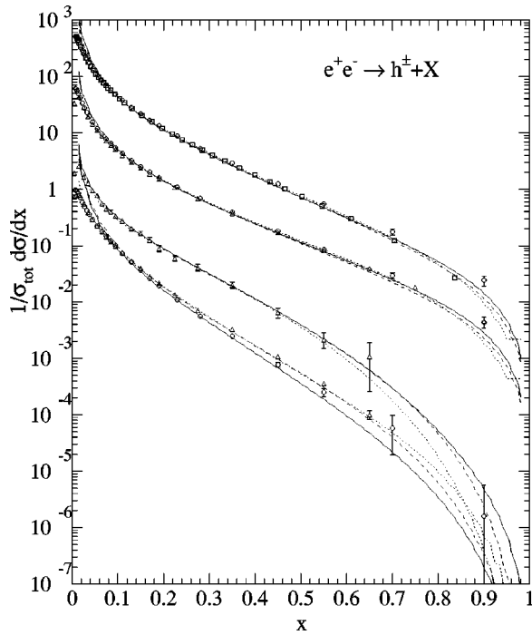
FIG. 26. Dependence of the normalized inclusive hadron cross section at \sqrt{s}=91.2 GeV on the scaled hadron momentum x . Data from DELPHI ( \Delta , 1991–1993; \circ , 1994; \square , SLD) are compared with the NLO fragmentation functions of Kniehl, Kramer, and Pötter (solid curve), Kretzer (dotted curve), and Bourhis, Fontannaz, et al. (dashed curve). Contributions from b , c , light, and all quarks (from bottom to top) are rescaled by factors of 1/5 relative to the nearest upper distribution. From Kniehl, Kramer, and Pötter, 2001.
