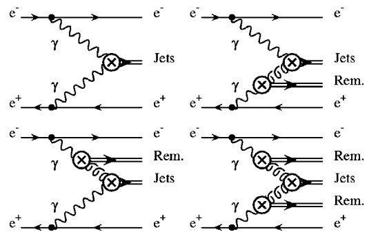
FIG. 5. Factorization of photon-photon scattering into jets.
