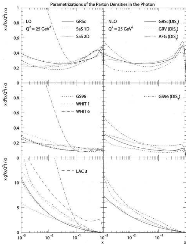
FIG. 2. Parametrizations of the up-quark (top), down-quark (center), and gluon (bottom) densities in the photon in leading order (LO; left) and next-to-leading order (NLO; right) at Q^2 = 25 \text{ GeV}^2 . The next-to-leading-order AFG and GS96 (Aurenche, Fontannaz, and Guillet, 1994a; Gordon and Storrow, 1997) parametrizations have been transformed from the \overline{\text{MS}} to the \text{DIS}_\gamma scheme.
