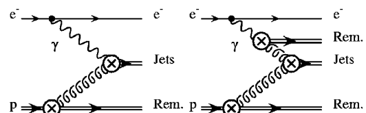
FIG. 6. Factorization of photon-hadron scattering into jets.
