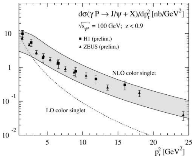
FIG. 44. J/\Psi transverse momentum distribution in leading-order (LO) and next-to-leading-order (NLO) direct color-singlet photoproduction. From Krämer, 2001.
