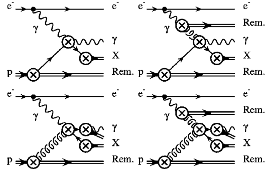
FIG. 47. Factorization of lepton-hadron scattering into photons.
