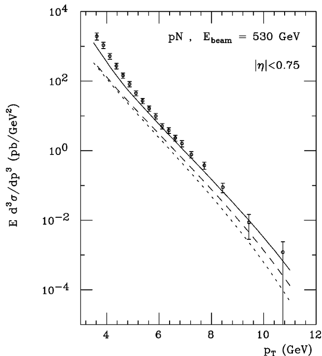
FIG. 60. Transverse momentum distribution of prompt photons produced in pN collisions at \sqrt{s} = 31.5 GeV: dotted curve, NLO; dashed curve, threshold resummed; solid curve, jointly resummed results are compared to E706 data (Laenen, Serman, and Vogelsang, 2000).
