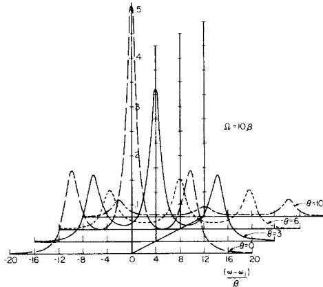
FIG. 7. Spectral density \Phi(\vec{r}, \omega)(\omega_0 \mu \sin \psi / 4 \pi \epsilon_0 c^2 \tau)^{-2} of the fluorescence at position \vec{r} in the long-time limit, for various detunings \theta = (\omega_1 - \omega_0 + \gamma) / \beta of the exciting field. The Rabi frequency \Omega = 10\beta . The elastically scattered \delta -function contribution is not shown.
